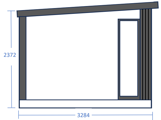
LH Side Elevation
