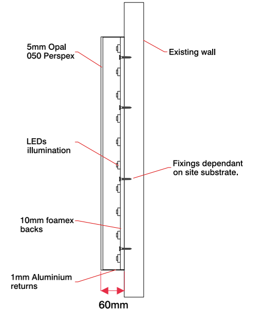
Section thru Scale 1:10
