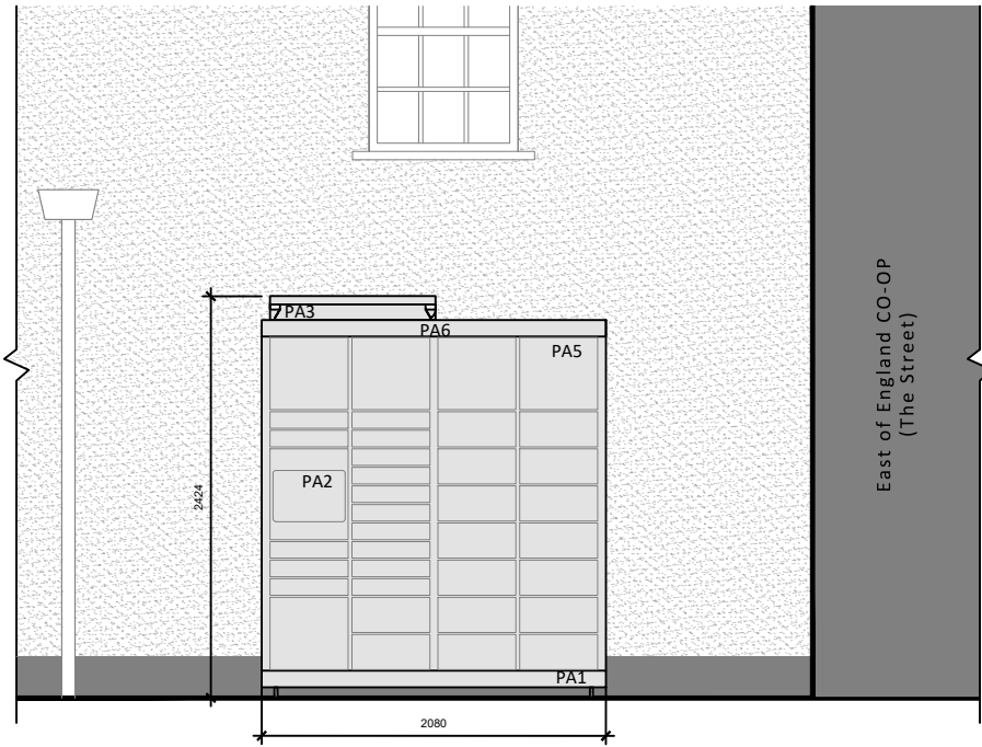
PROPOSED ELEVATION A SCALE 1:50
