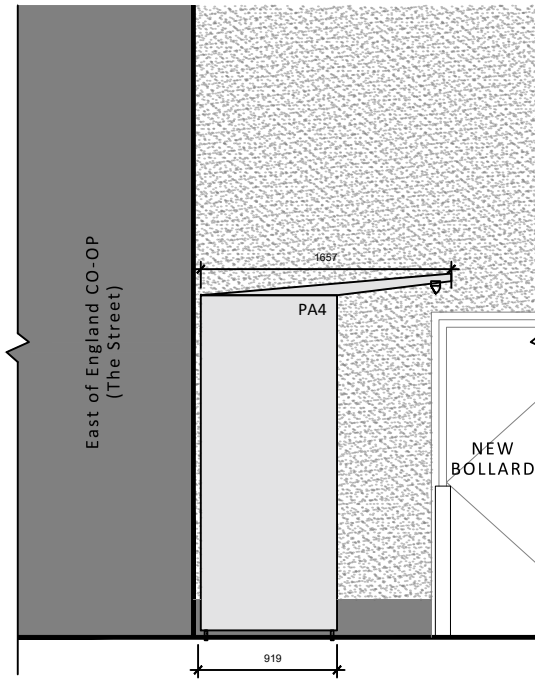
PROPOSED ELEVATION B SCALE 1:50
