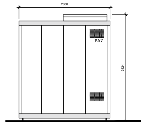
PROPOSED ELEVATION D SCALE 1:50
