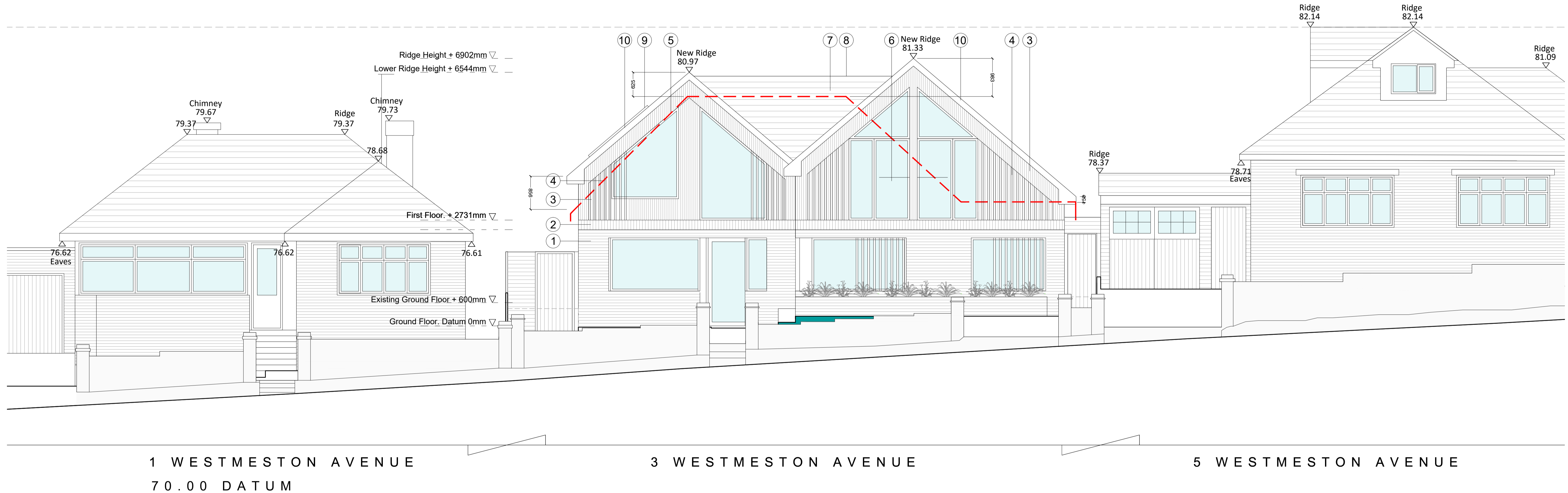
01 Front Elevation - East Scale: 1:50
