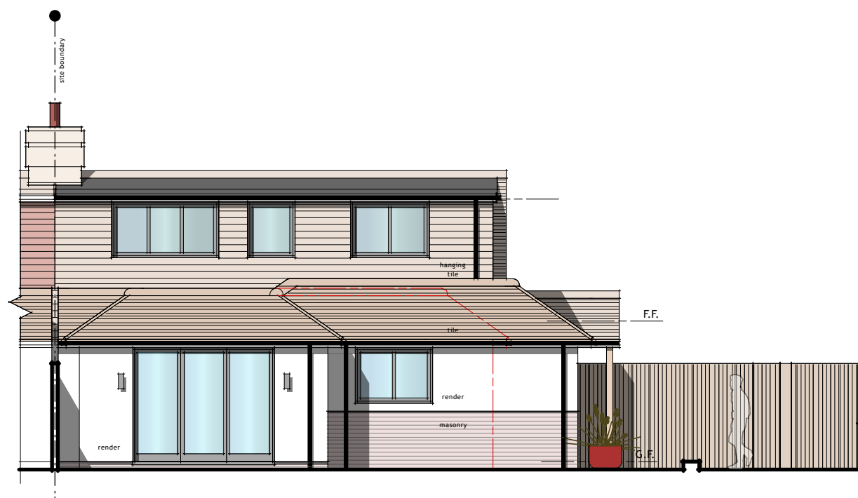
REAR ELEVATION 2
