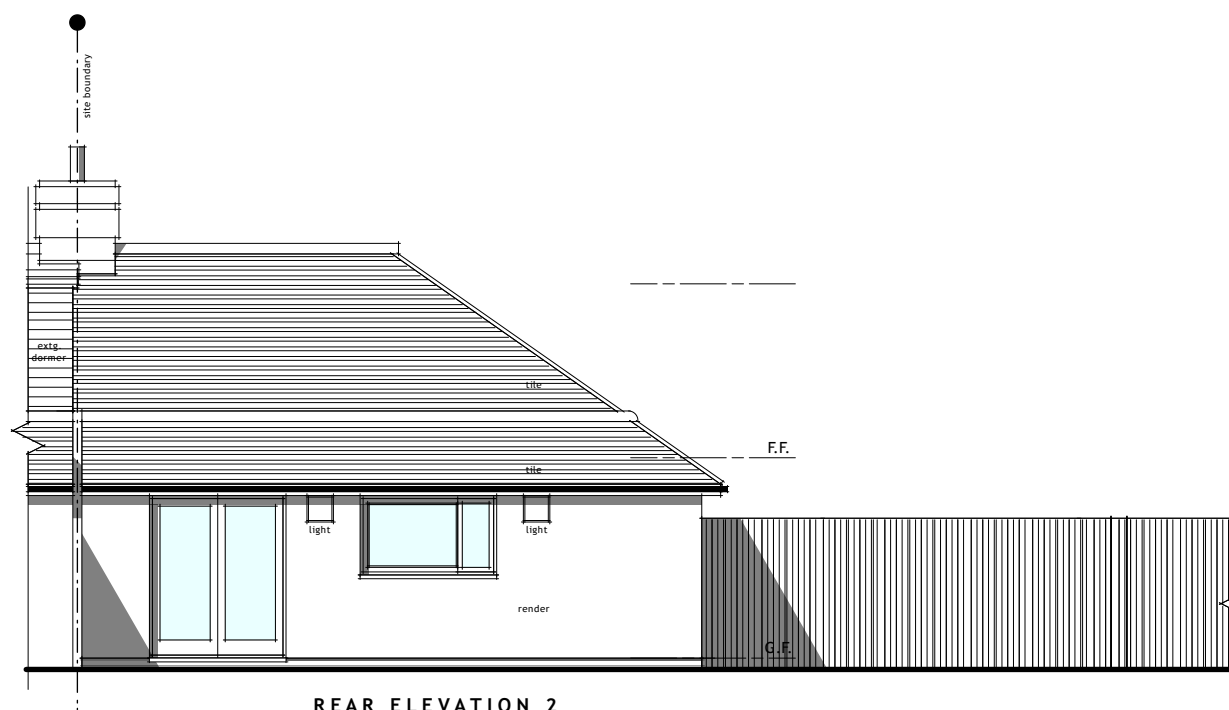
REAR ELEVATION 2
