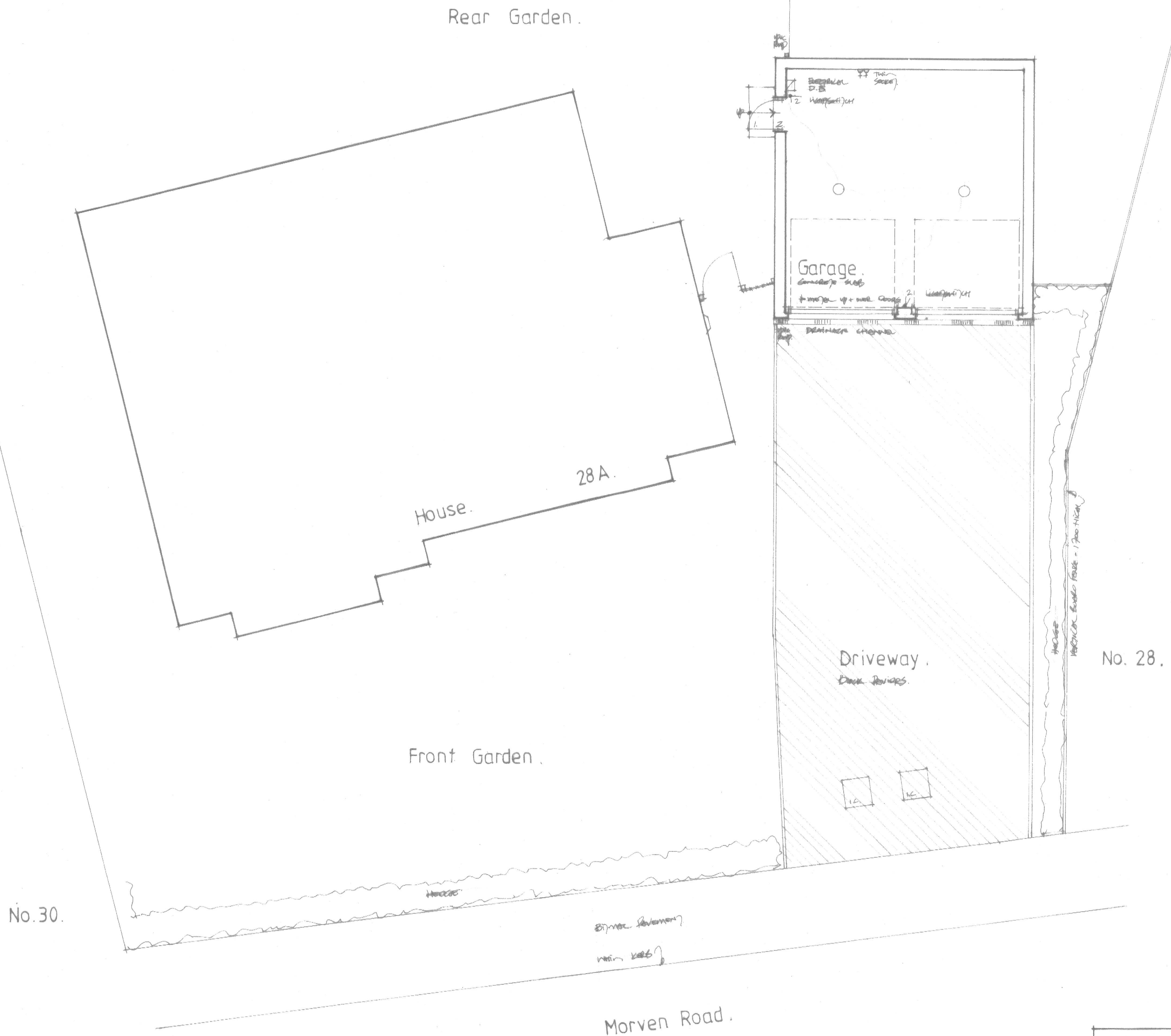
Part Site Plan / Ground Floor Plan of Garage as Existing . 1:50.
