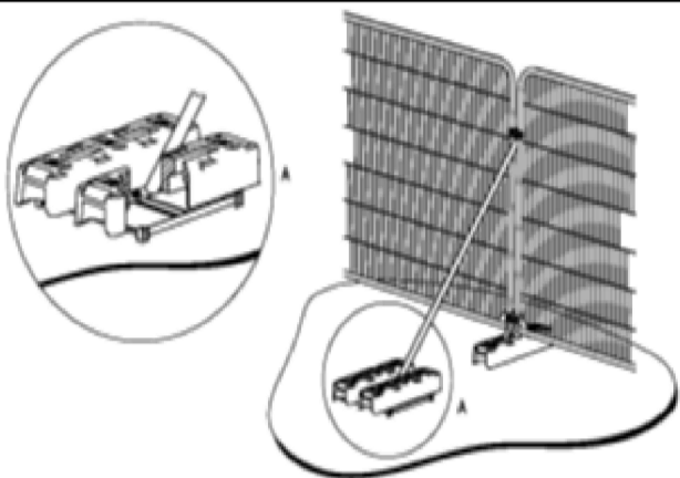
b) Stabilizer strut mounted on block tray
