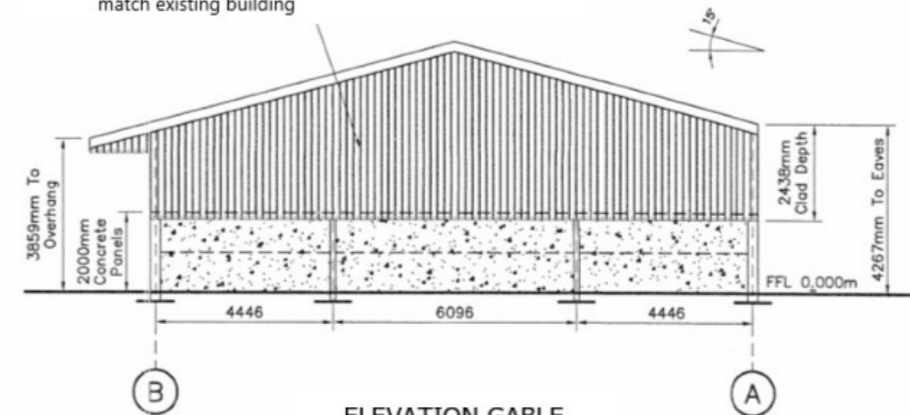
ELEVATION GABLE 1:100
