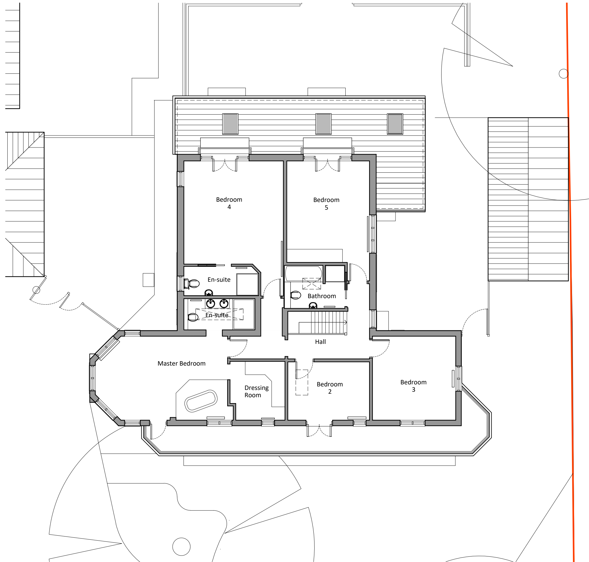
Existing First Floor Plan 1:100
