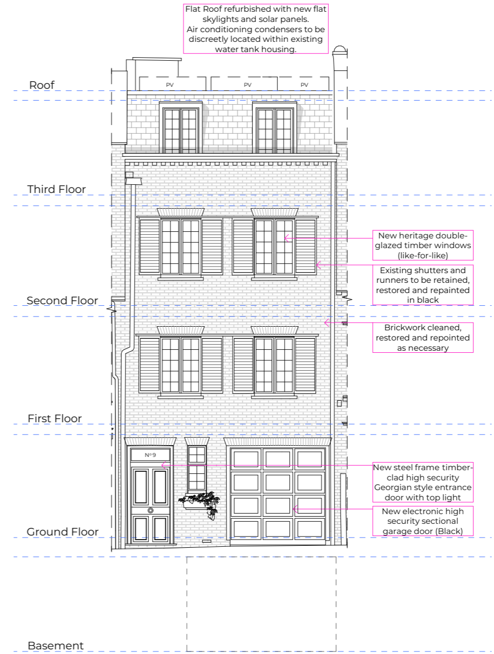
Proposed Front Elevation 9 Mount Row
