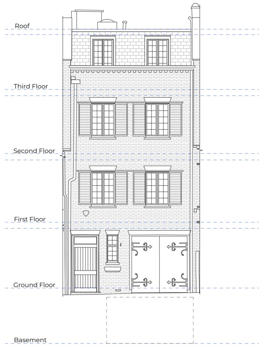
Existing Front Elevation 9 Mount Row
