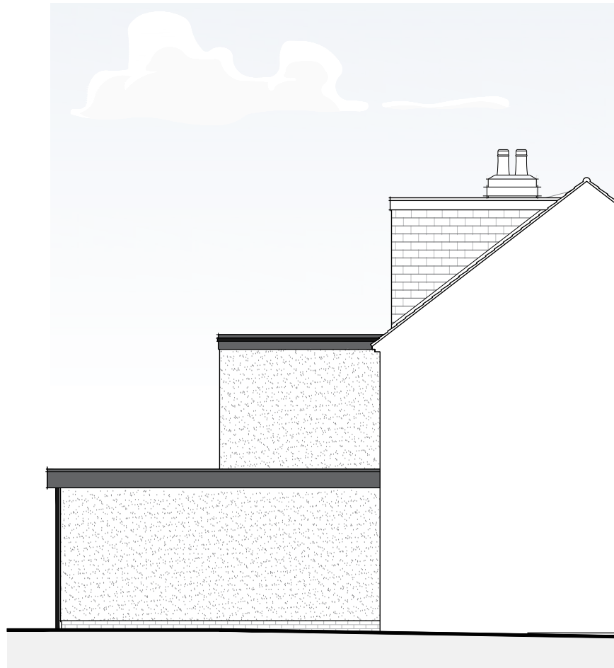
East Elevation
