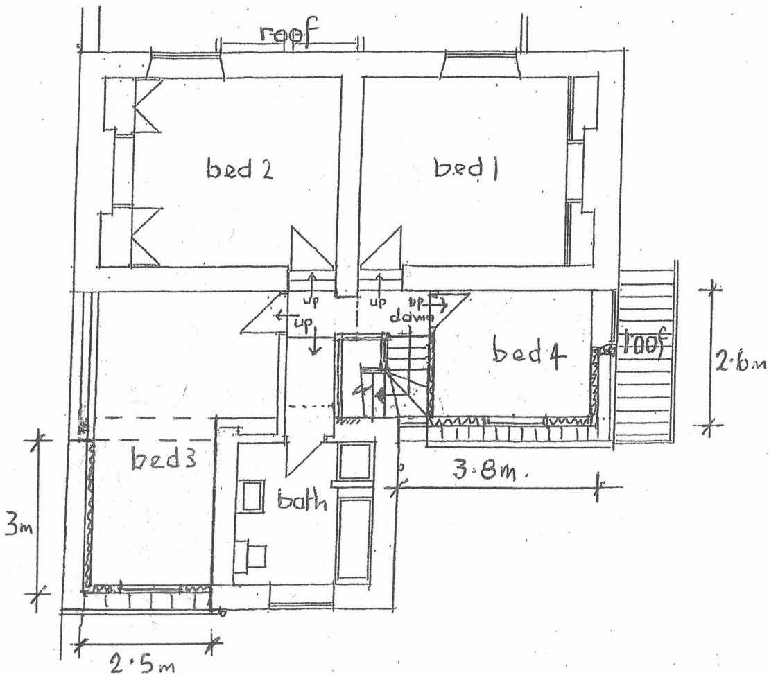
First Floor Plan 1:100 As Proposed
