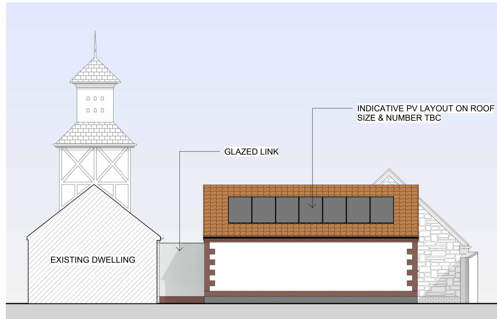
West Elevation 1 : 100
