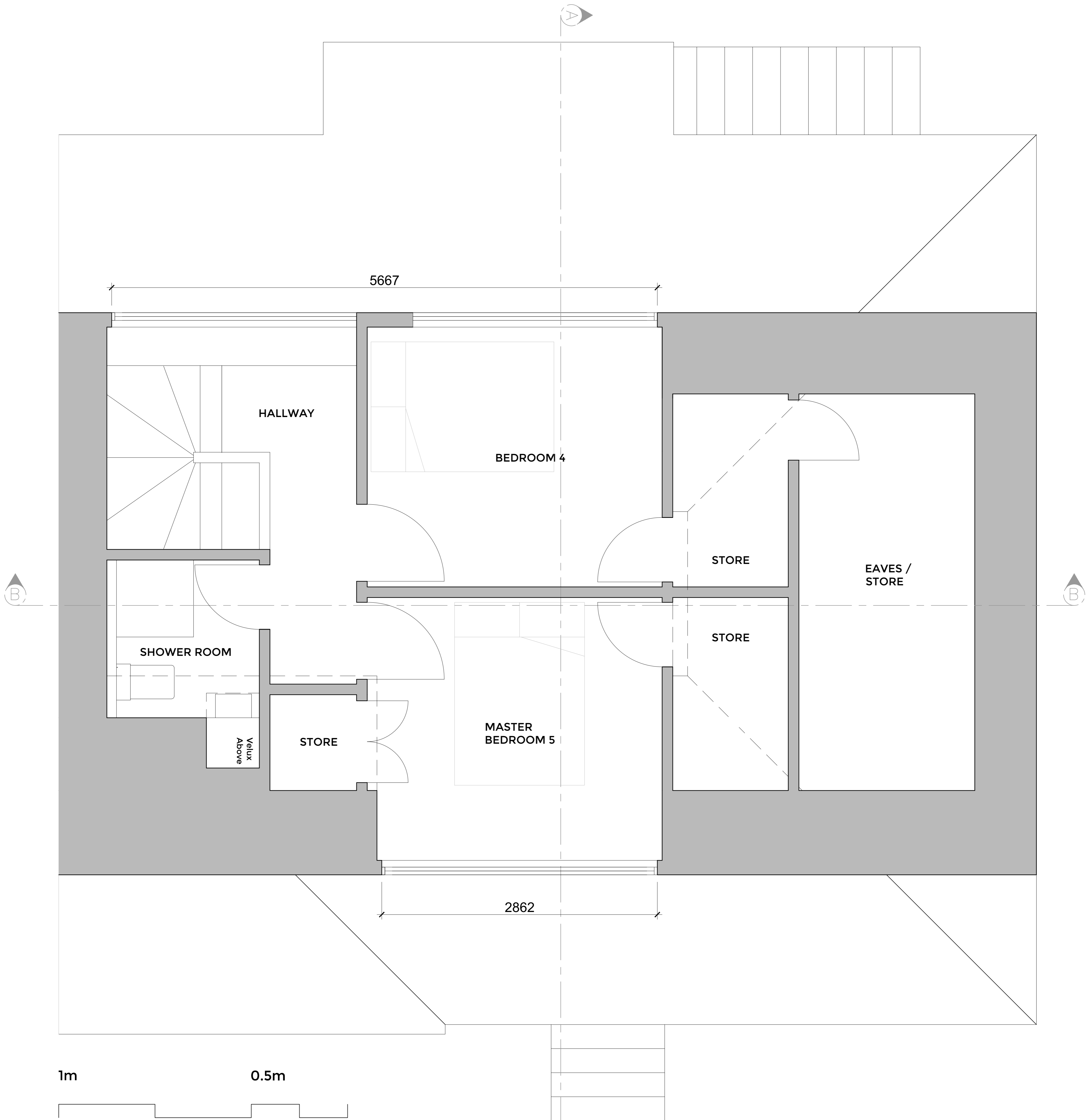
ATTIC FLOOR PLAN AS PROPOSED
