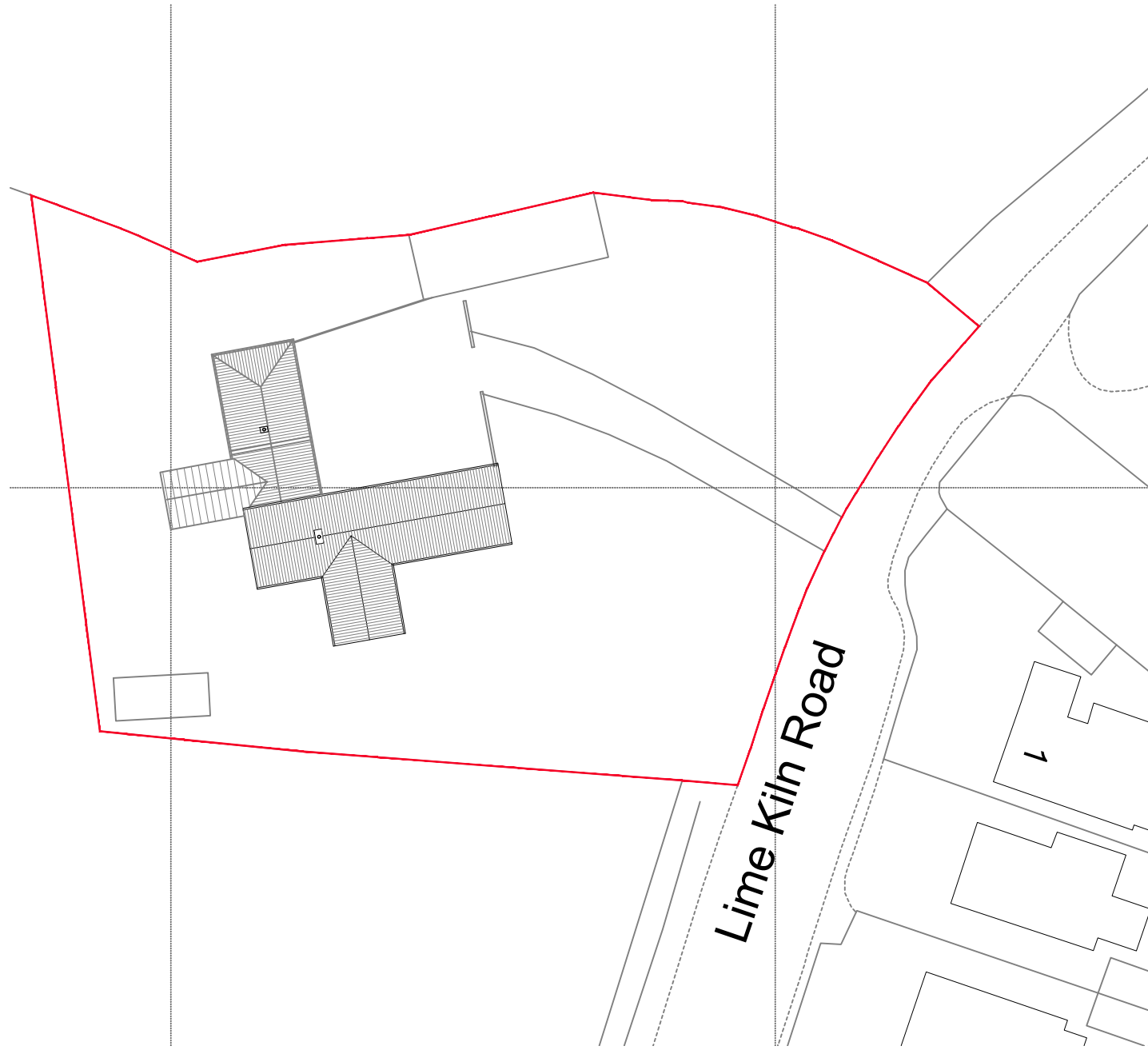
A EXISTING SITE & ROOF PLAN 002 SCALE 1:500
