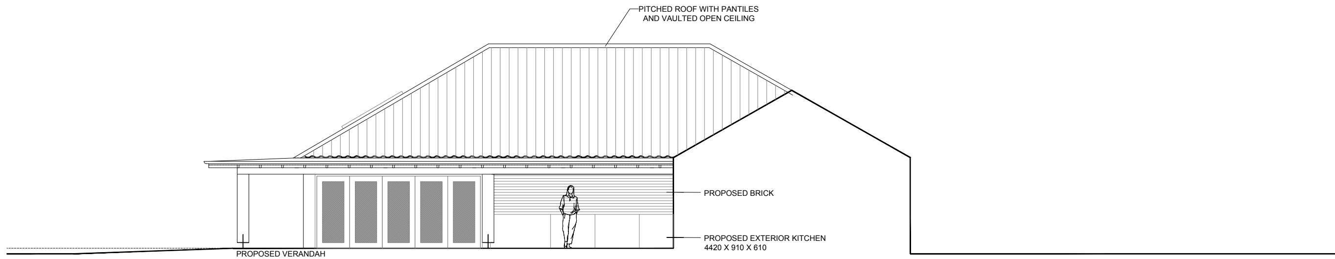
A PROPOSED SOUTH ELEVATION + PARTIAL 008 BUILDING SECTION THROUGH COURTYARD - SCALE 1:100
