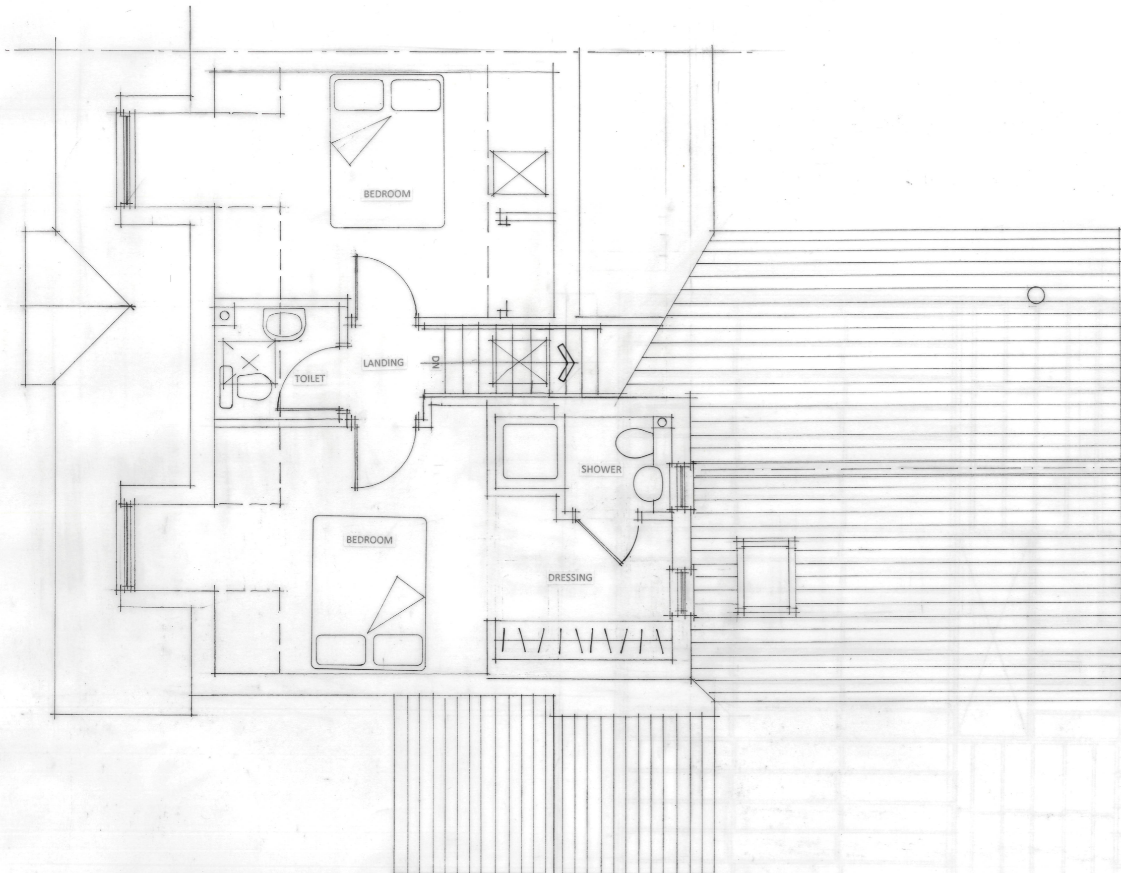
1:50 FIRST FLOOR PLAN AS PROPOSED
