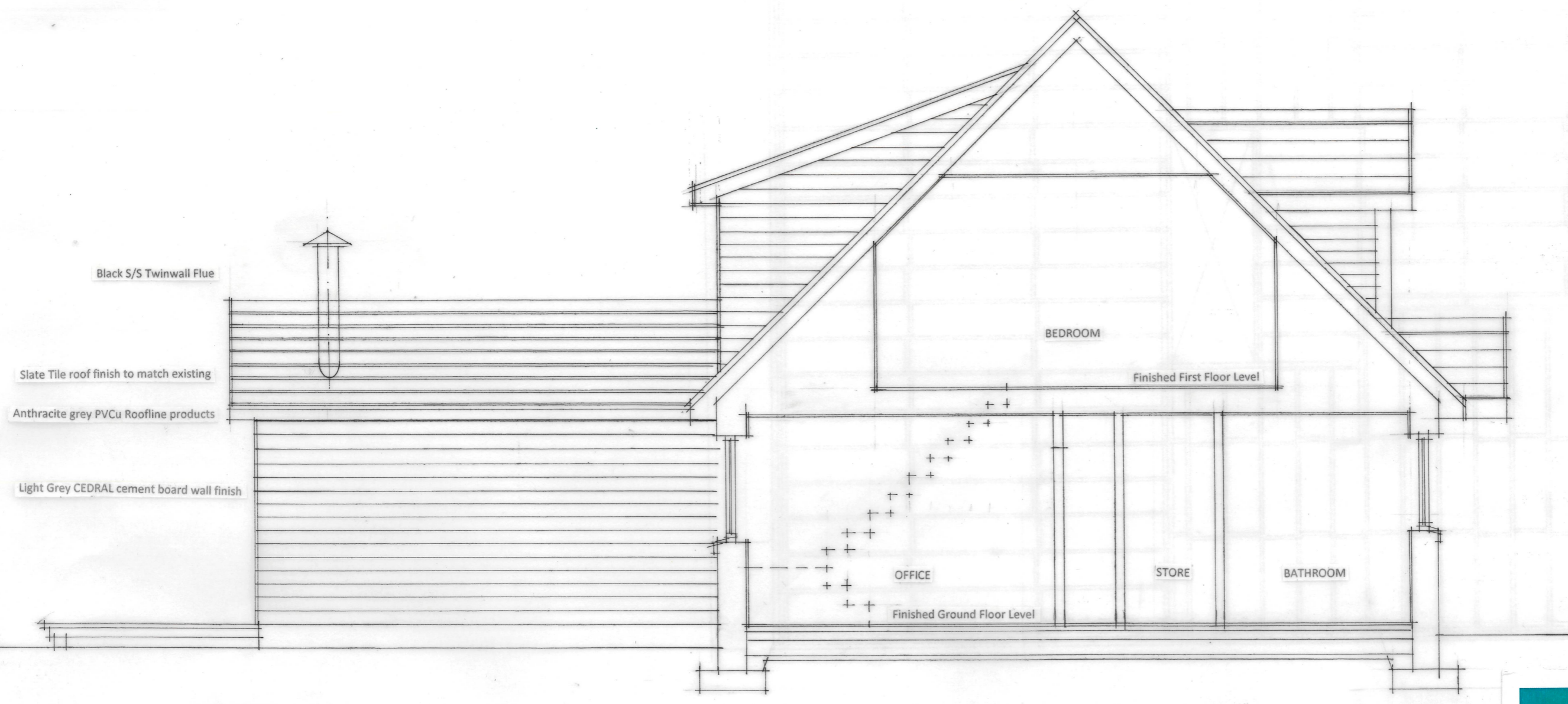
1:50 SIDE (EAST) ELEVATION & SECTION AS PROPOSED
