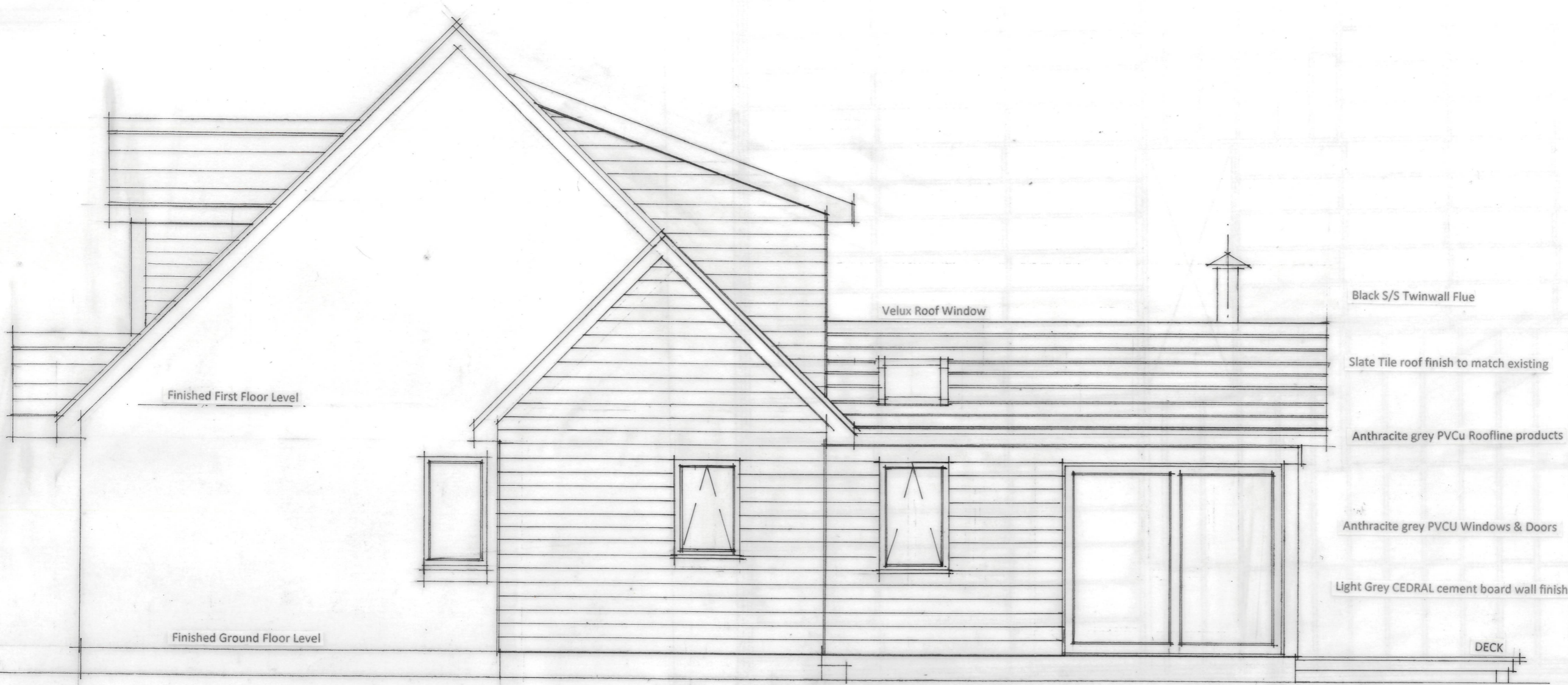
1:50 SIDE (WEST) ELEVATION AS PROPOSED
