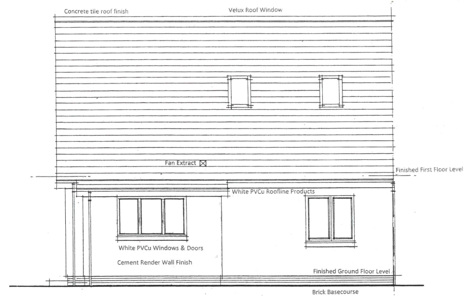
1:100 REAR ( SOUTH) ELEVATION AS EXISTING
