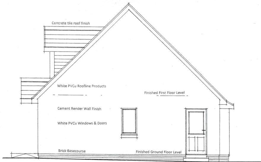
1:100 SIDE (WEST) ELEVATION AS EXISTING
