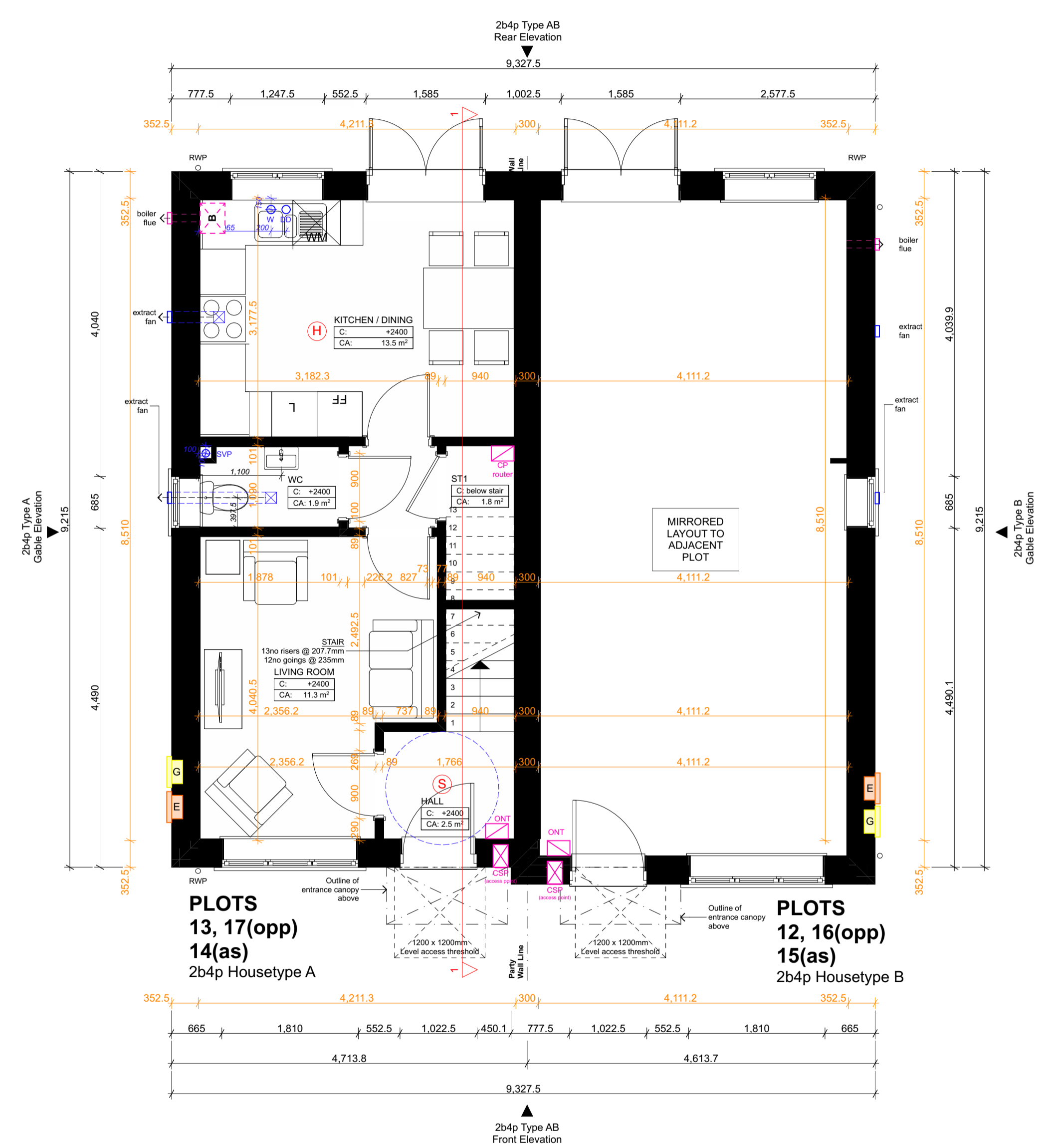
2b4p Type AB House type pair - GROUND FLOOR BLOCK PLAN 1:50
