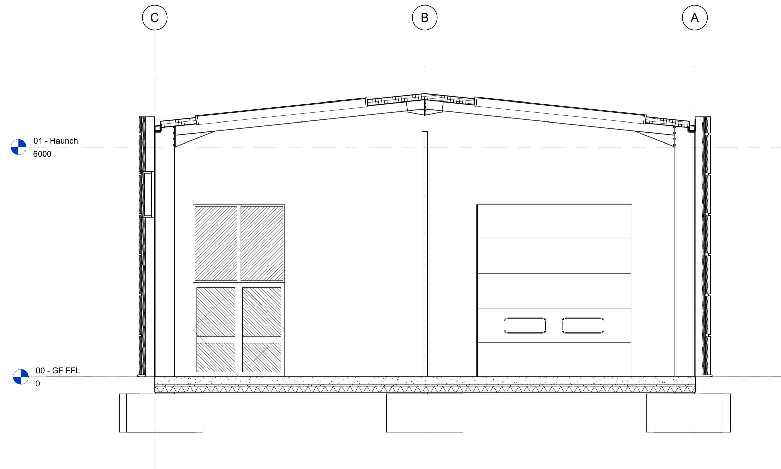
1 Proposed GA Section 1 : 50
