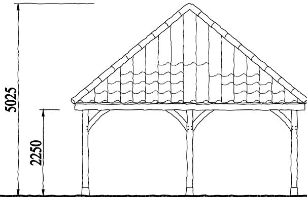
Side Elevation
