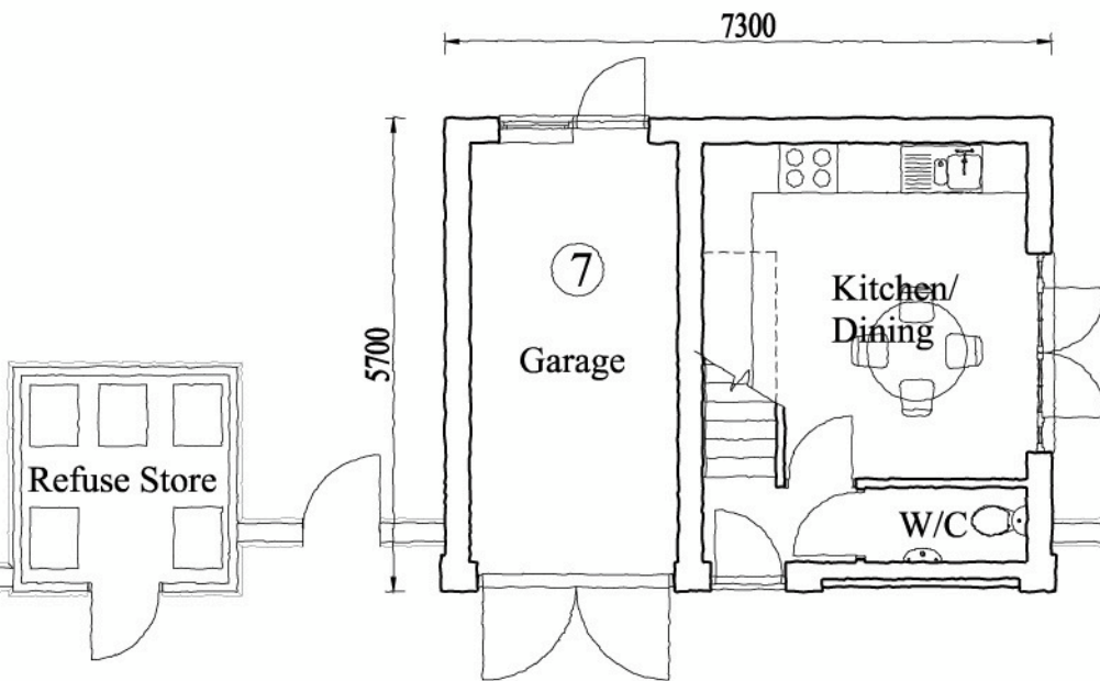
Ground Floor Plan 54m 2
