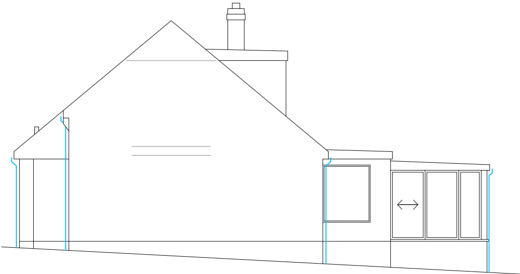
EXISTING RIGHT SIDE ELEVATION
