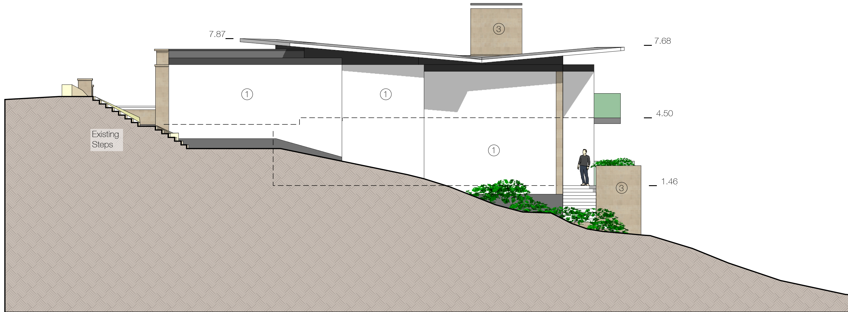
NORTH WEST ELEVATION AS PROPOSED 1:100 @ A3
