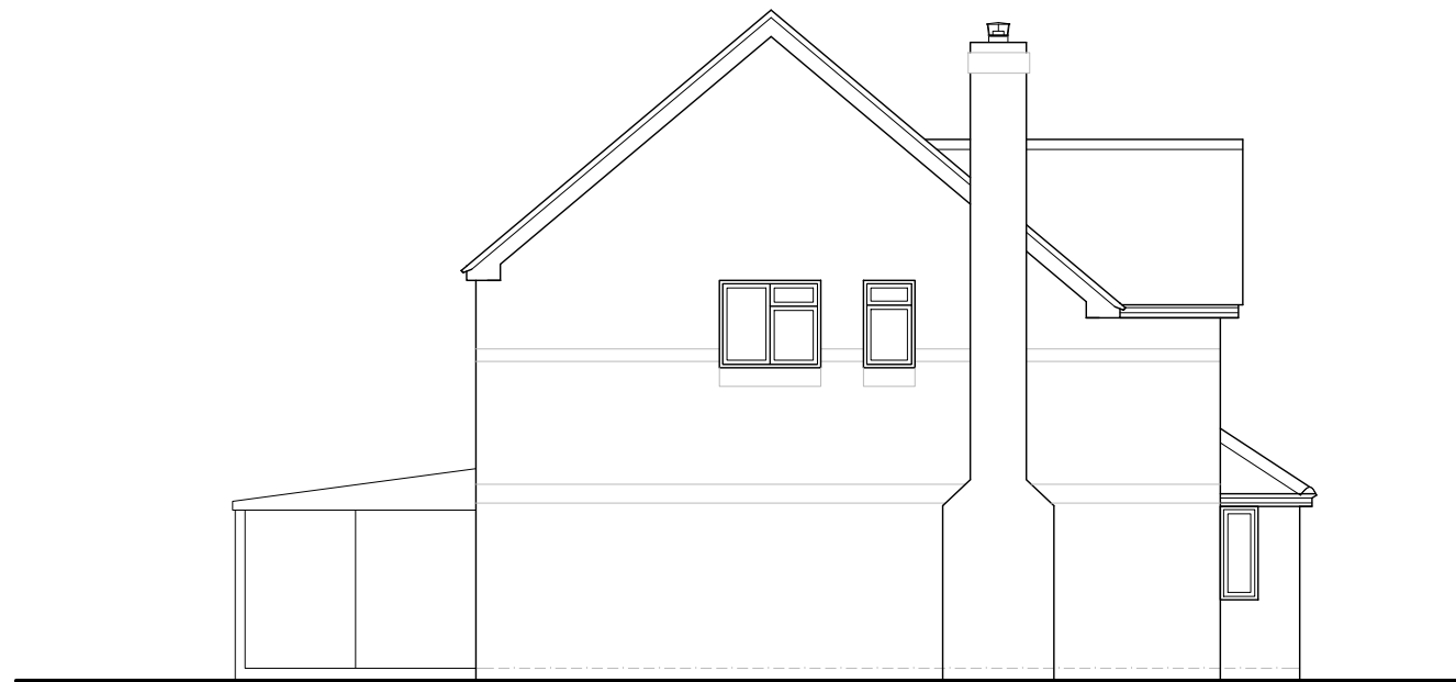
South (side) Elevation | existing
