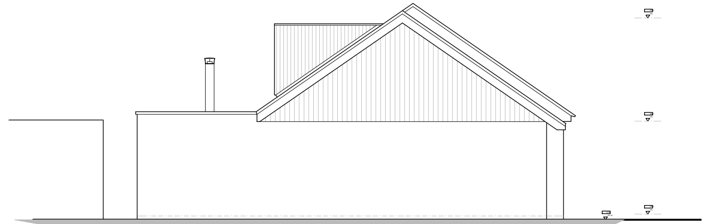
East Elevation | proposed
