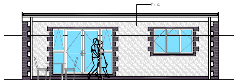
Proposed Front (North) Elevation
