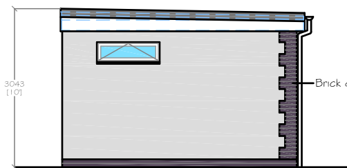
Proposed Side (East) Elevation
