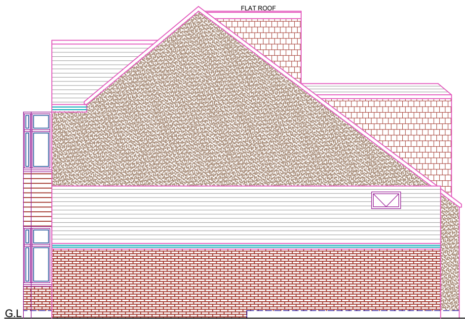
PROPOSED ELEVATION SIDE A
