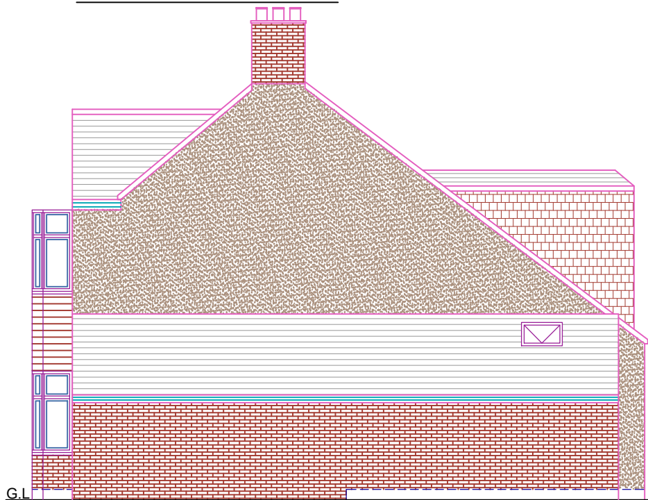
EXISTING ELEVATION SIDE A
