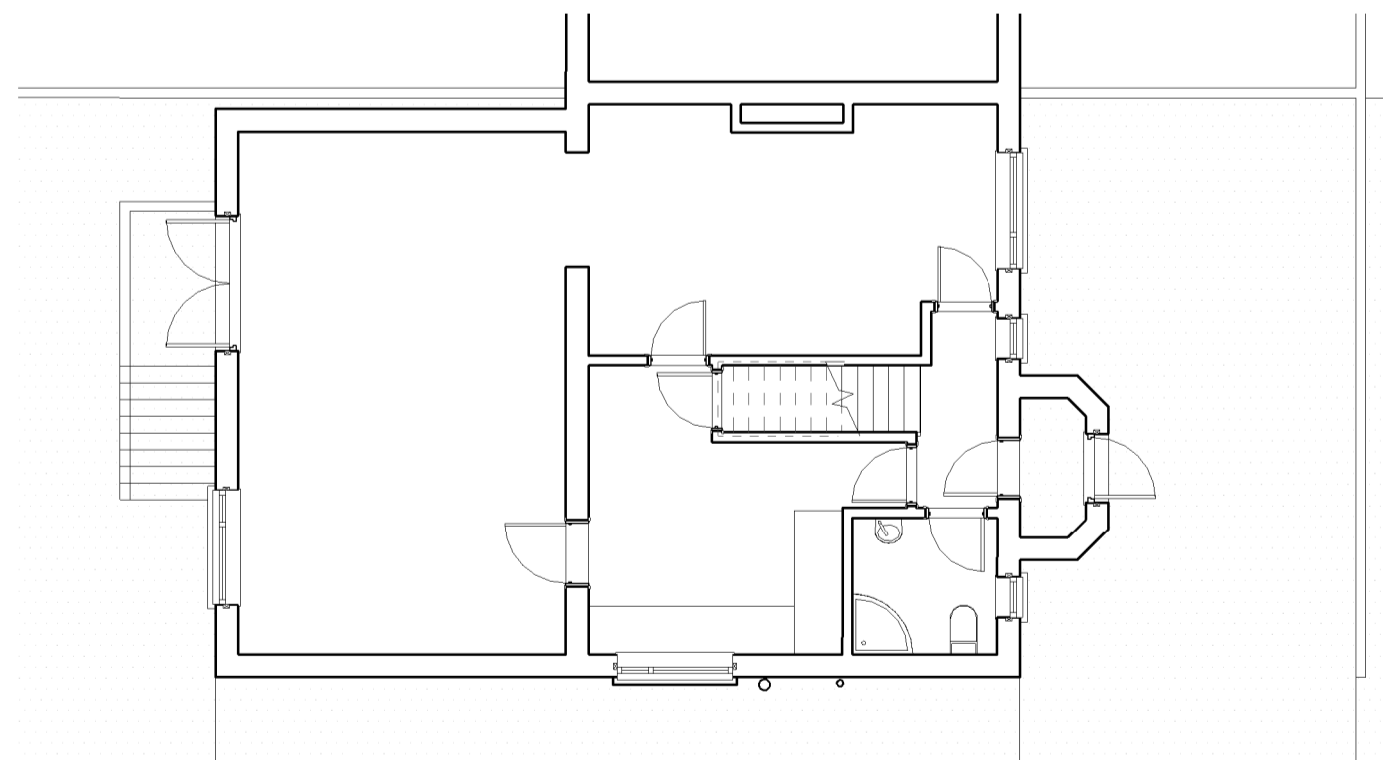
4 GROUND FLOOR PLAN SCALE: 1 : 100
