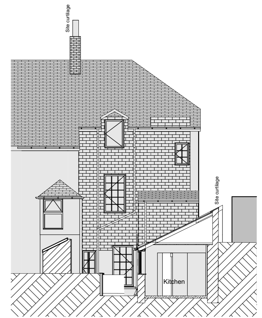
4 As Existing Rear/North Elevation (03) 1:100
