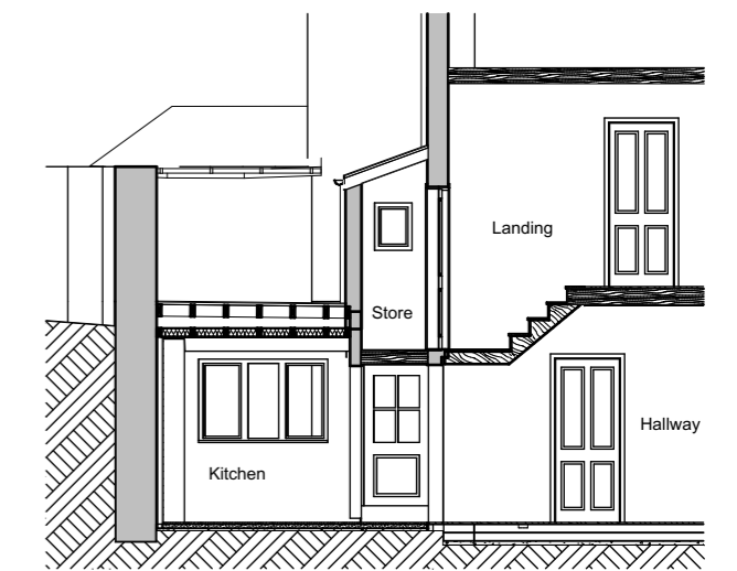
6 As Existing Section 2 1:100
