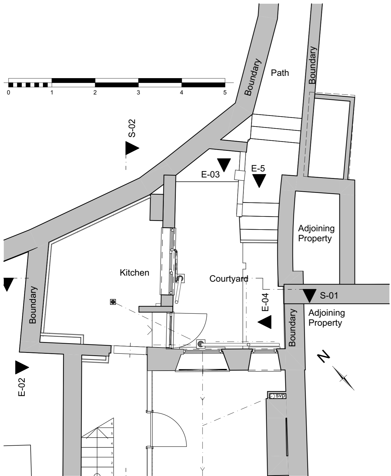
1 GF-Ground Floor 1:50
