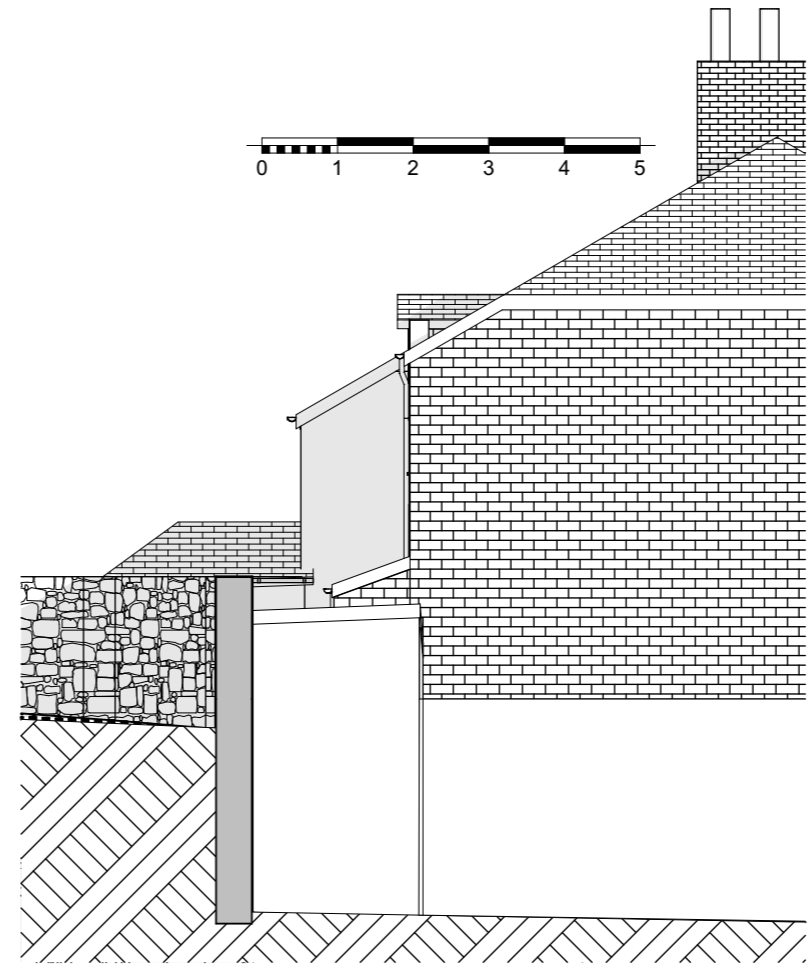
3 As Existing Side/West Elevation (02) 1:100
