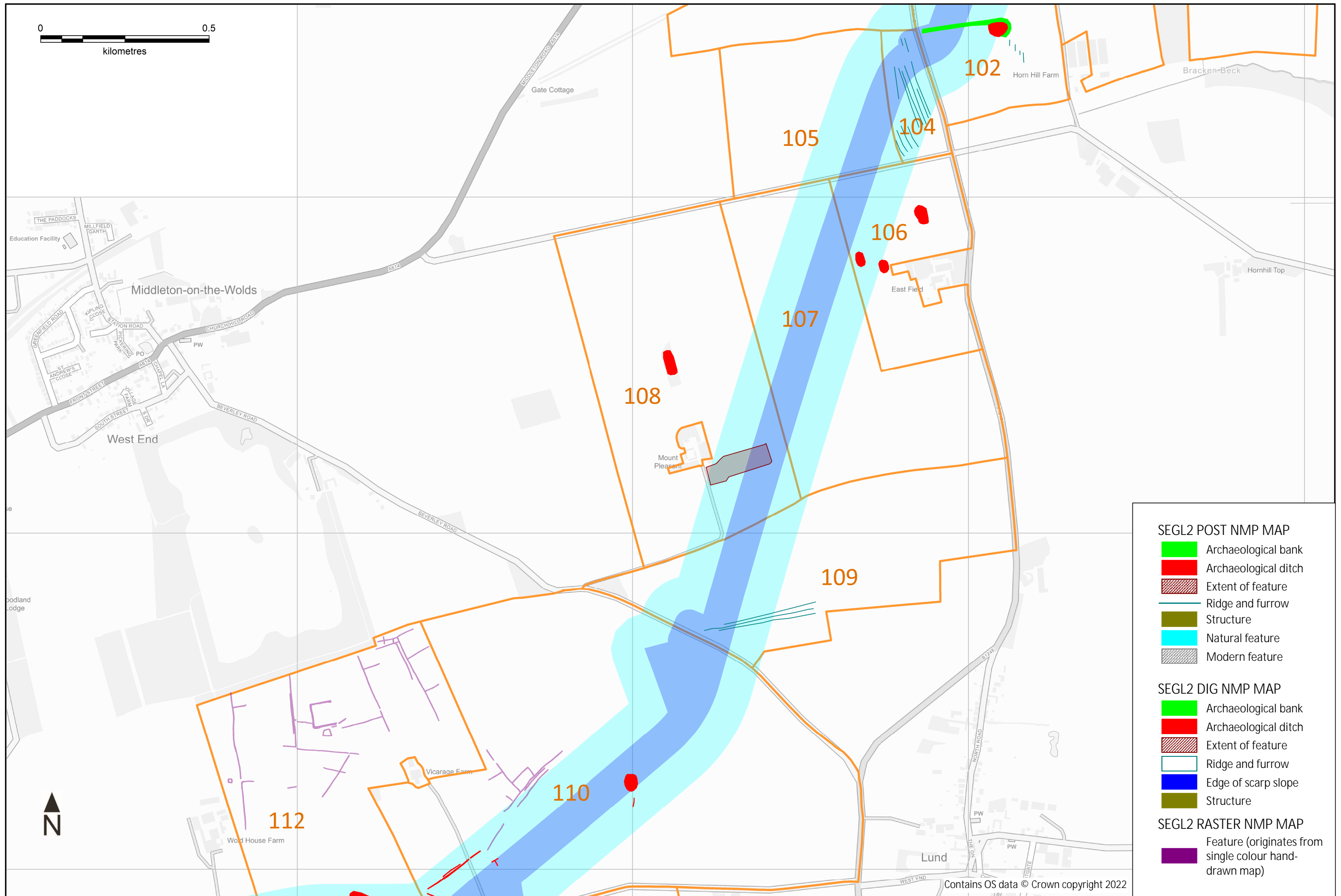
Figure 9 Overview of LiDAR and air photo mapping for the Scotland England Green Link – SEGL2 (fields 102 to 112)
