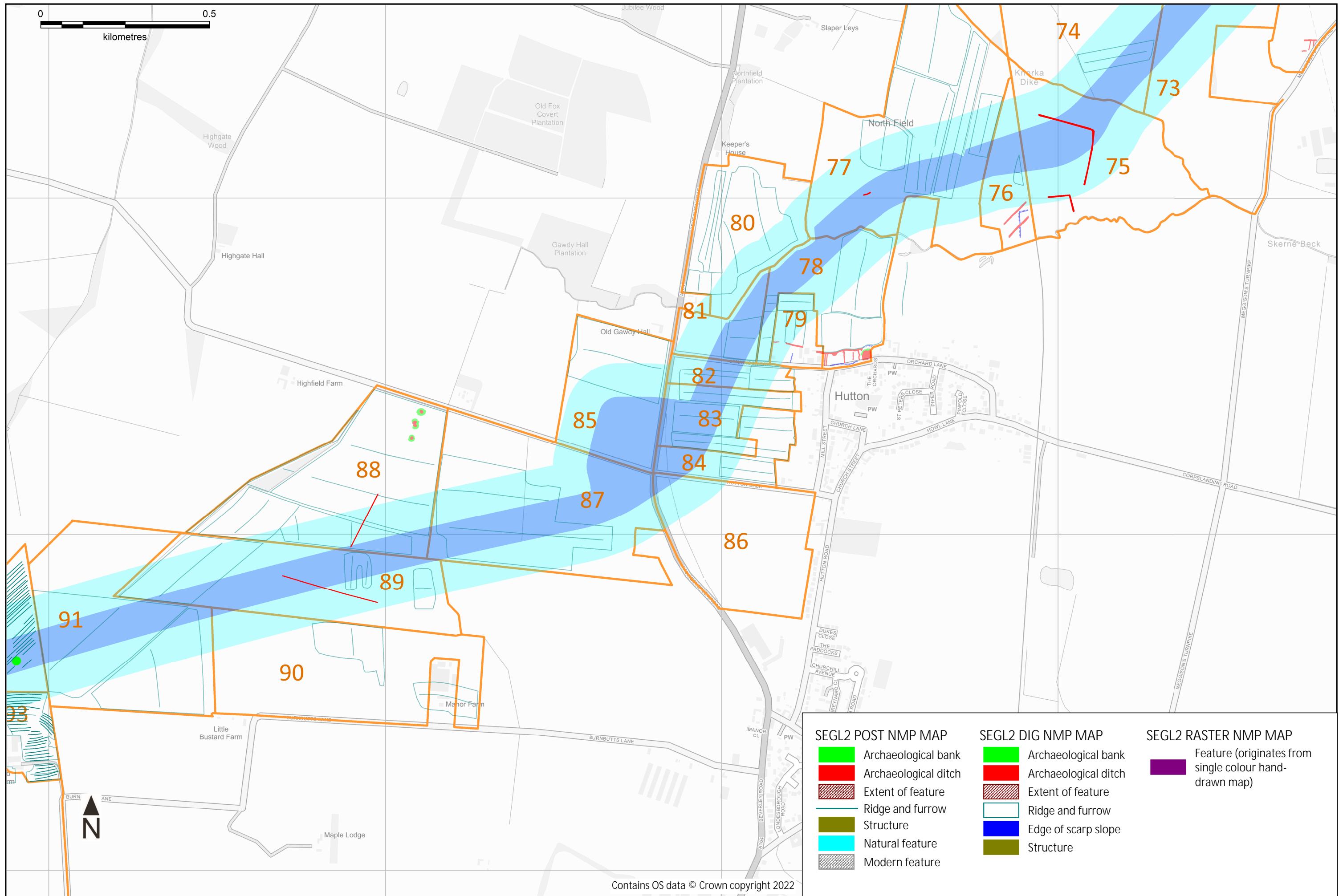
Figure 7 Overview of LiDAR and air photo mapping for the Scotland England Green Link – SEGL2 (fields 73 to 91)
