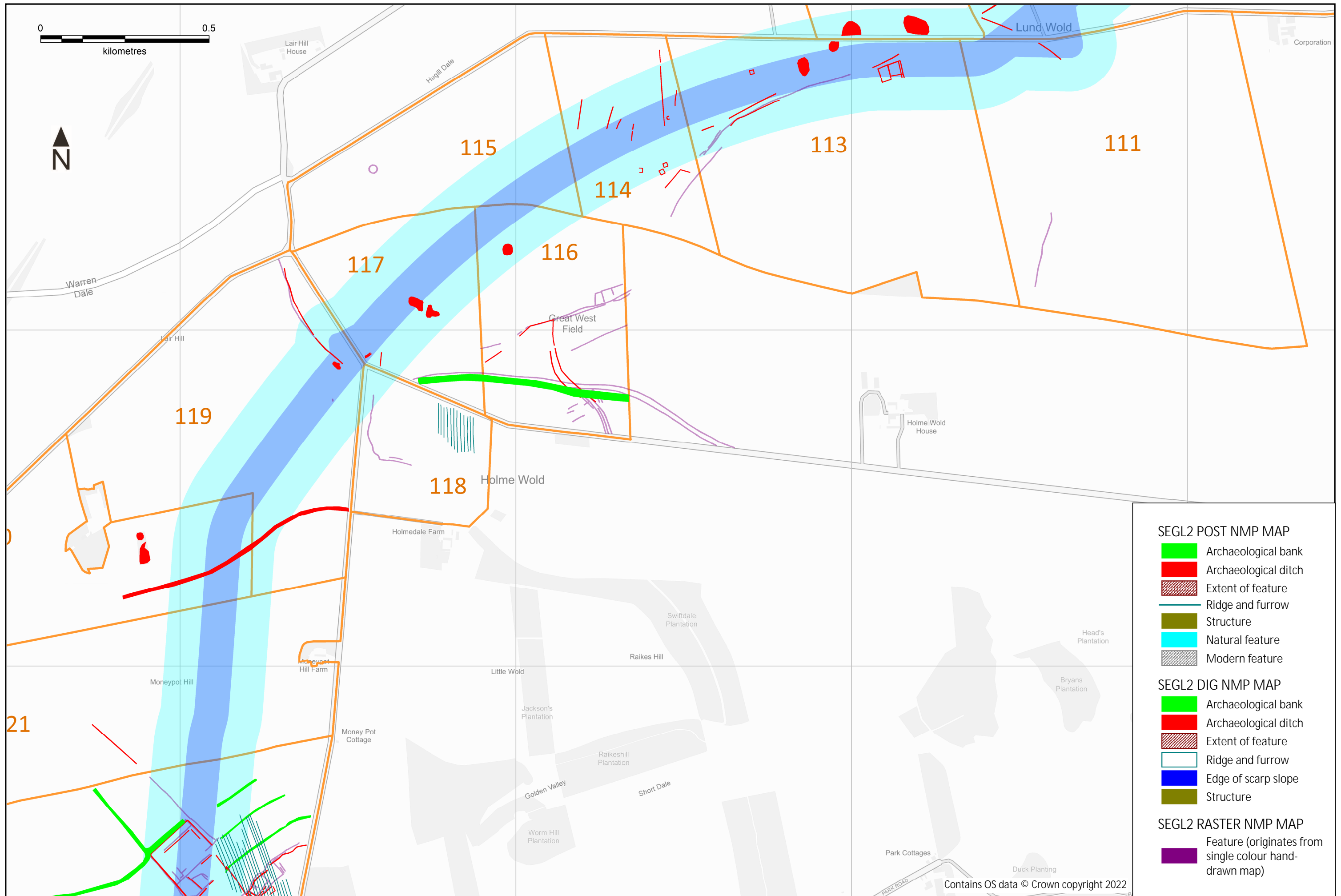
Figure 10 Overview of LiDAR and air photo mapping for the Scotland England Green Link – SEGL2 (fields 111 to 119)
