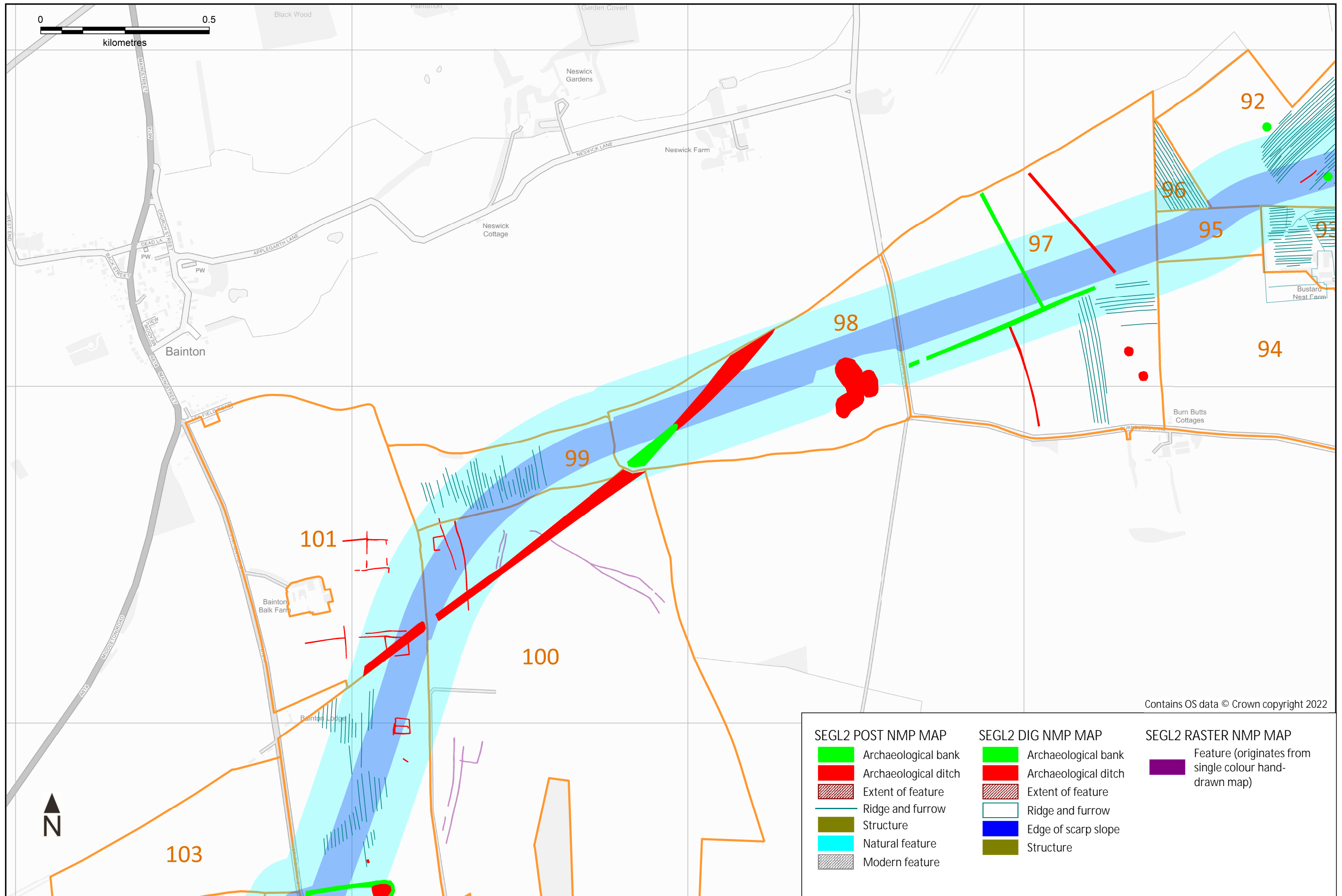
Figure 8 Overview of LiDAR and air photo mapping for the Scotland England Green Link – SEGL2 (fields 92 to 103)
