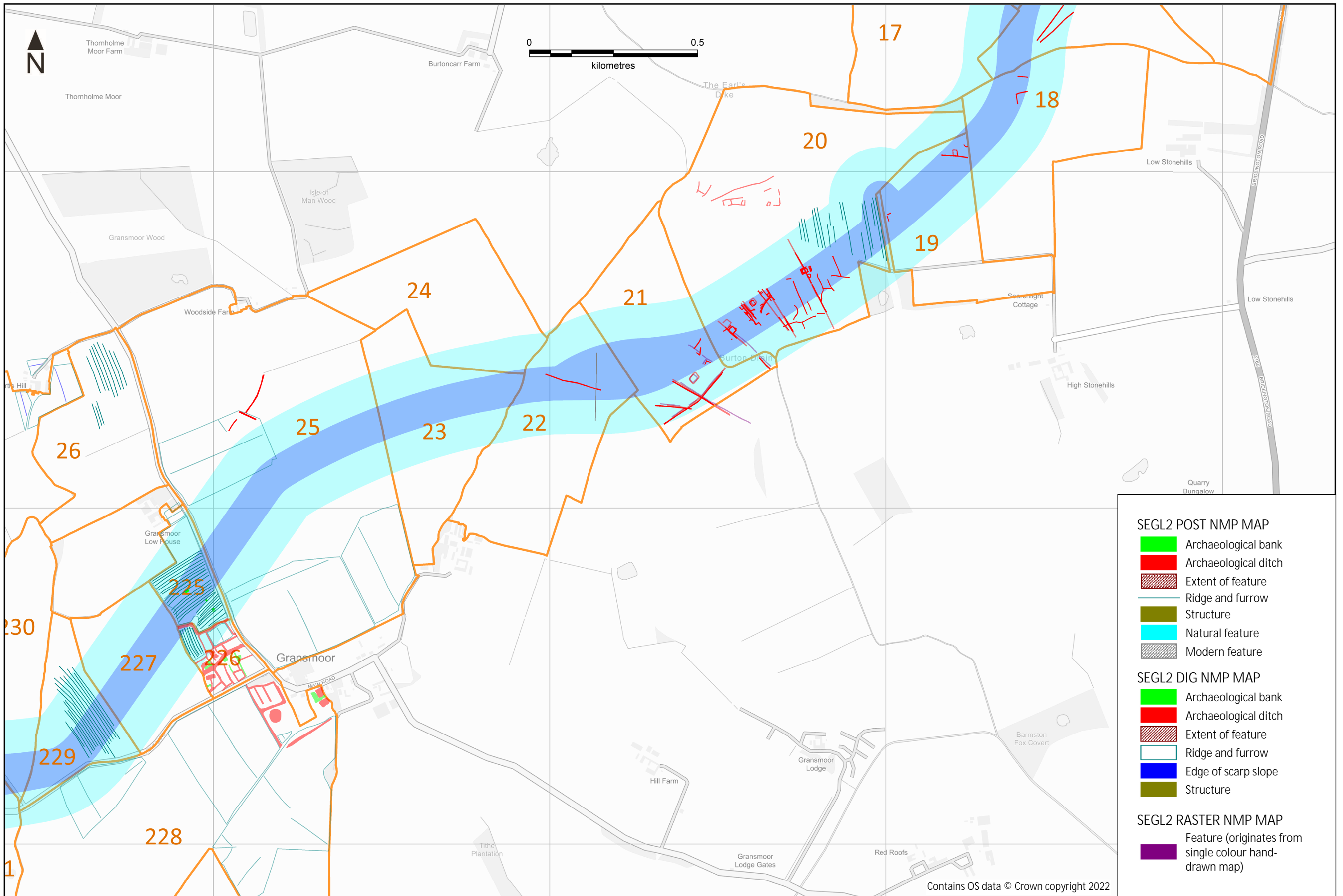
Figure 3 Overview of LiDAR and air photo mapping for the Scotland England Green Link – SEGL2 (fields 17 to 26 and 225 to 229)
