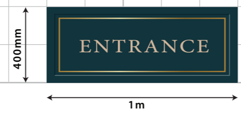
E ONE X NEW TRANSOM PANEL SIZE. 1m x 400mm. H.A.G. 2m.
