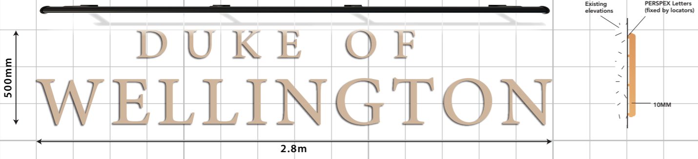
B ONE X NEW SET OF INDIVIDUAL LETTERS AND NEW TROUGH LIGHT SIZE. 2.8m x 500mm. H.A.G. 2.5m.
