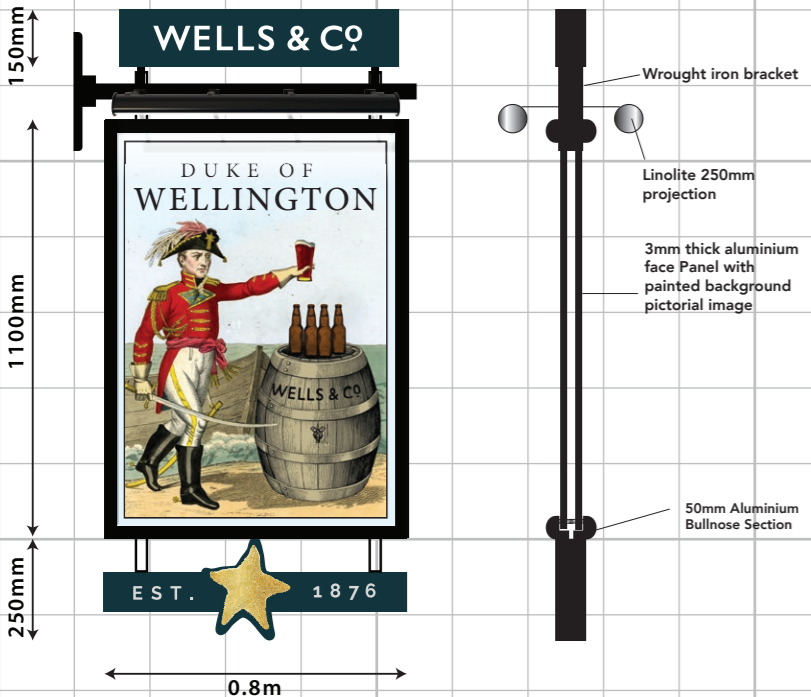
C ONE X NEW COMPLETE PICTORIAL INCLUDING HEADER, FOOTER AND LIGHTING TO EXISTING POST SIZE. 0.8m x 1100mm. H.A.G. 4.3m.
