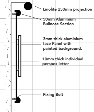
G ONE X NEW GABLE BOARD. ONE X NEW TROUGH LIGHT SIZE. 2.7m x 1400mm. H.A.G. 3.4m.
