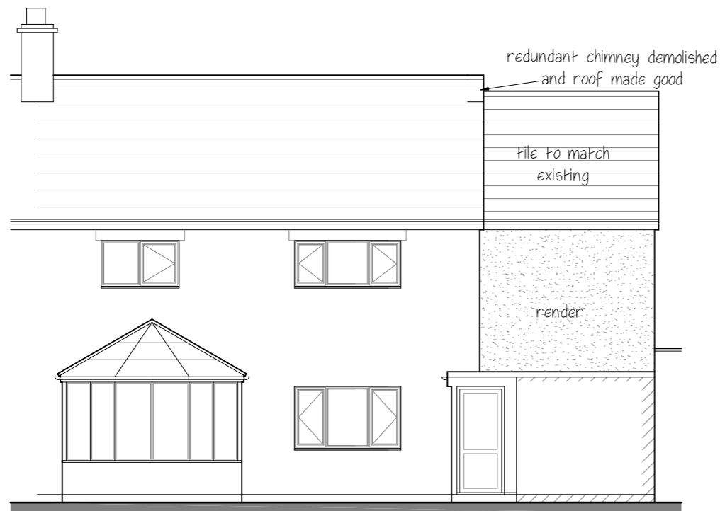
rear elevation
