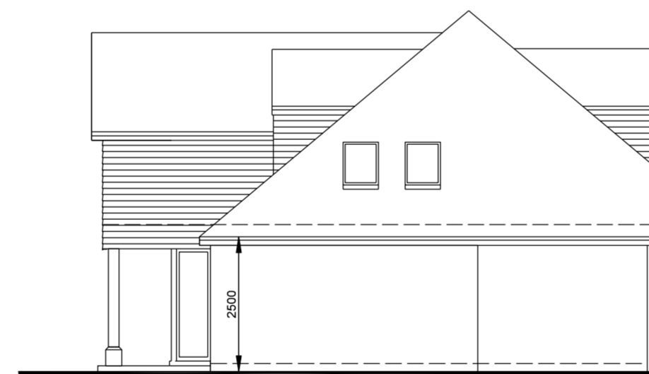
West Elevation
