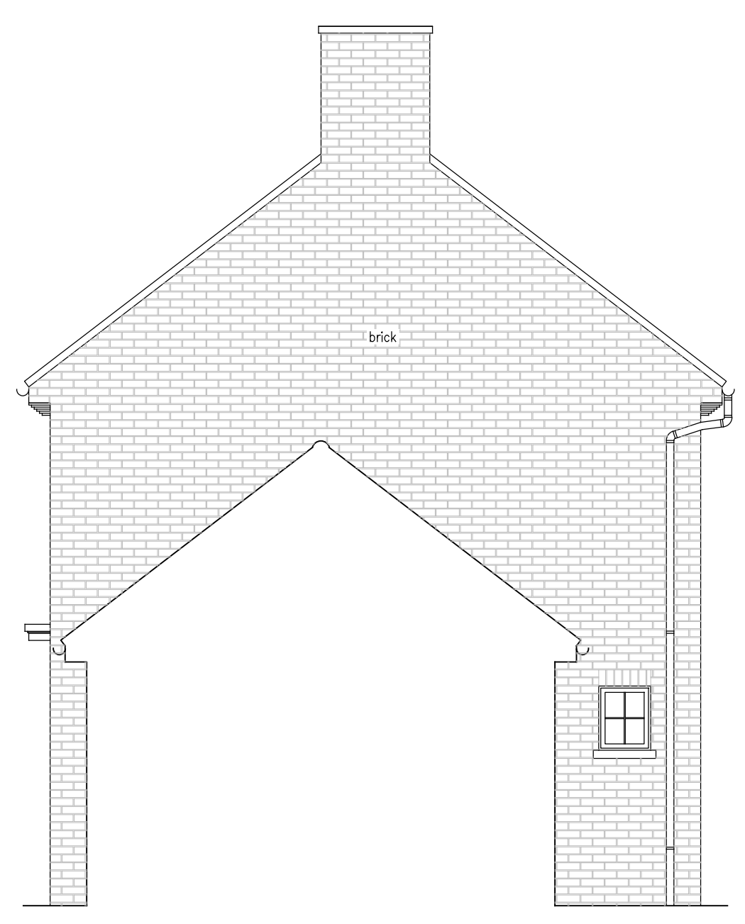
existing right side elevation 1:50
