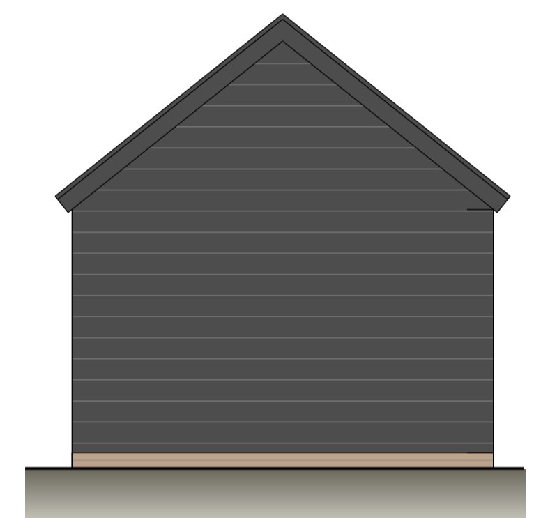
PROPOSED ELEVATION (west)
