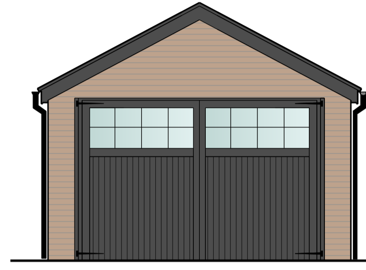
PROPOSED ELEVATION (northeast)
