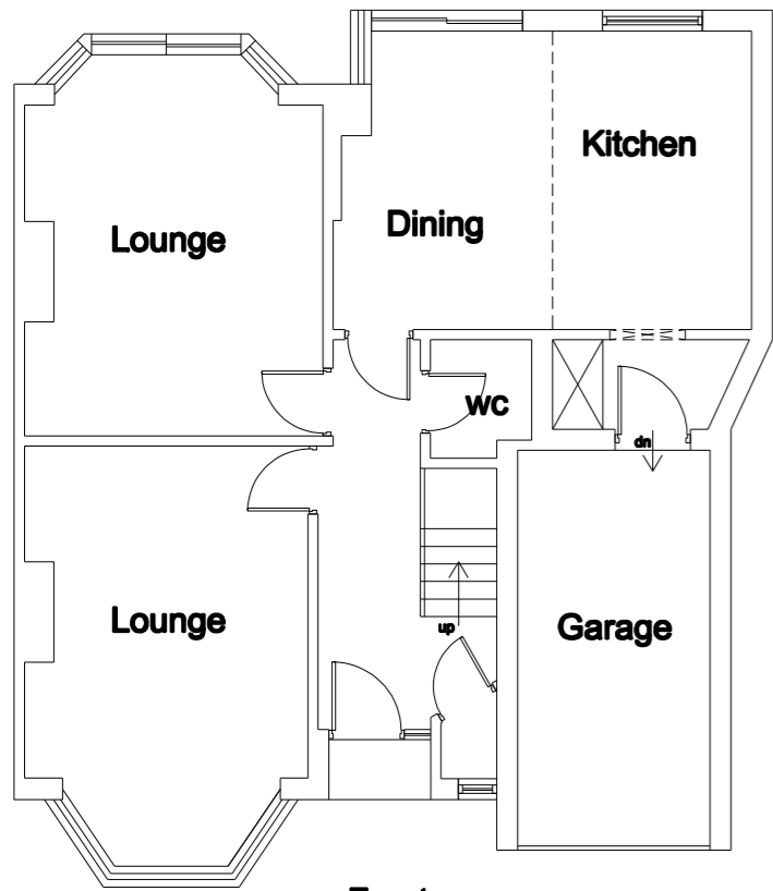
Front Existing Ground Floor Plan
