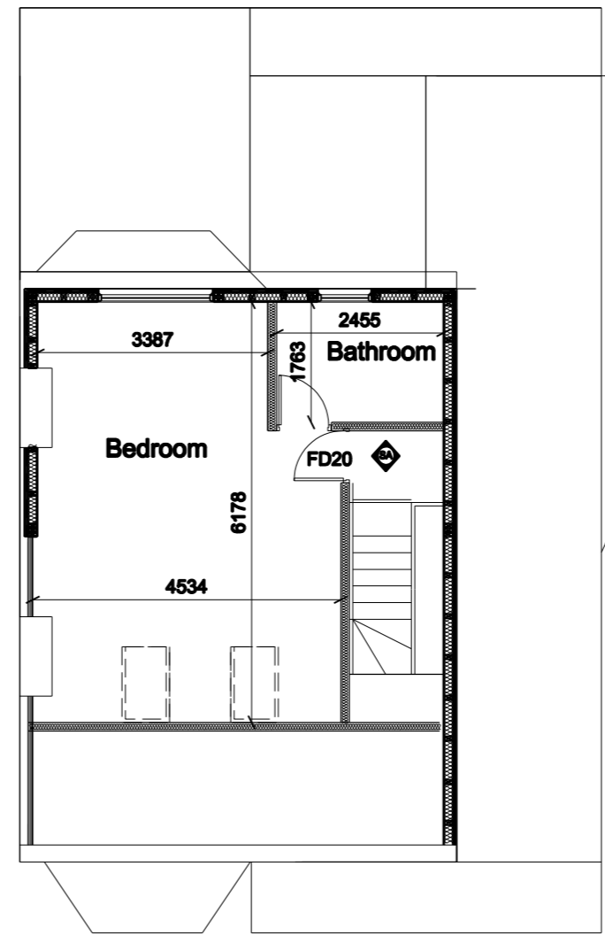
Proposed Loft Plan
