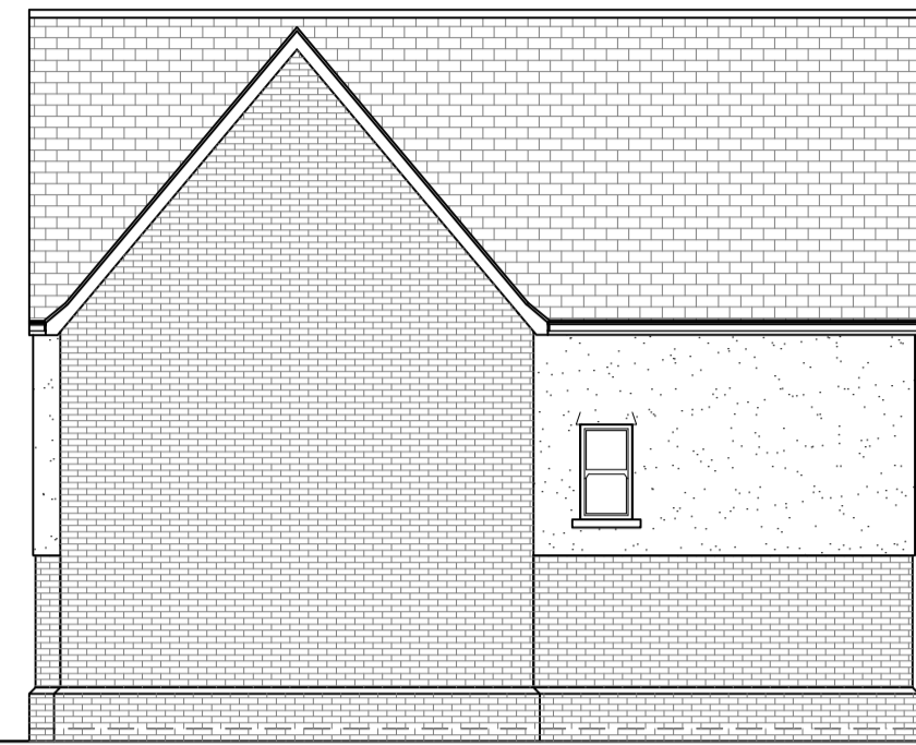
SIDE ELEVATION (1:100)
