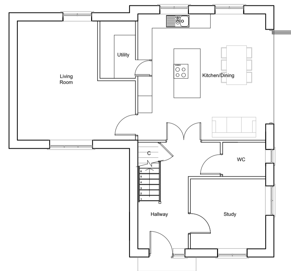
GROUND FLOOR PLAN PLOT 07 FLOOR AREA - 180m 2 4 BED / 7 PERSON
