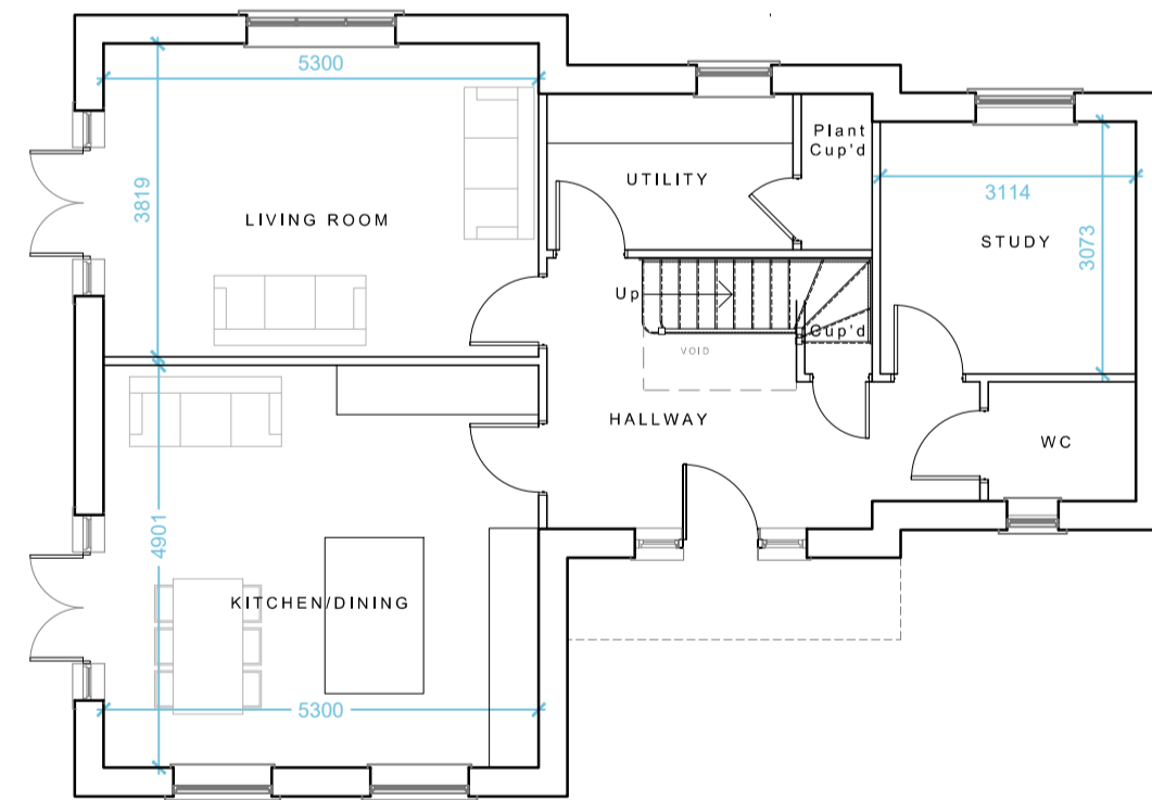
GROUND FLOOR PLAN PLOT 01 FLOOR AREA - 185m 2 4 BED / 7 PERSON
