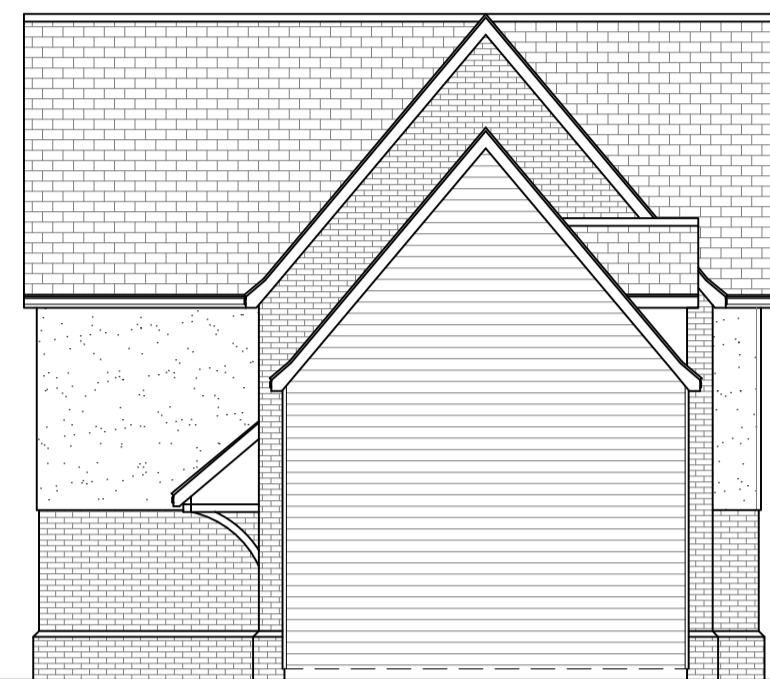
SIDE ELEVATION (1:100)
