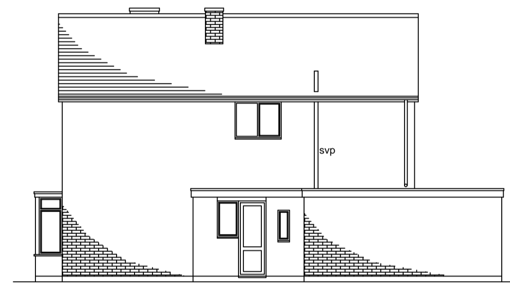
EXISTING ADJ. SIDE ELEVATION (scale 1:100)
