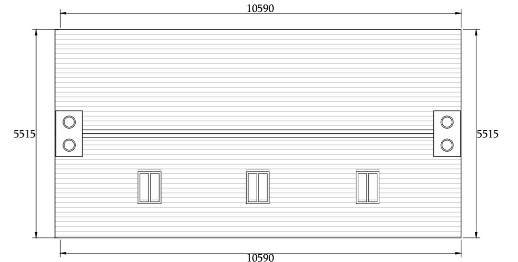
ROOF PLAN 1:100
