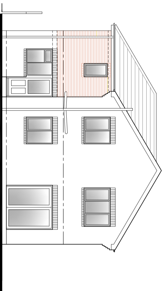
SOUTH ELEVATION
