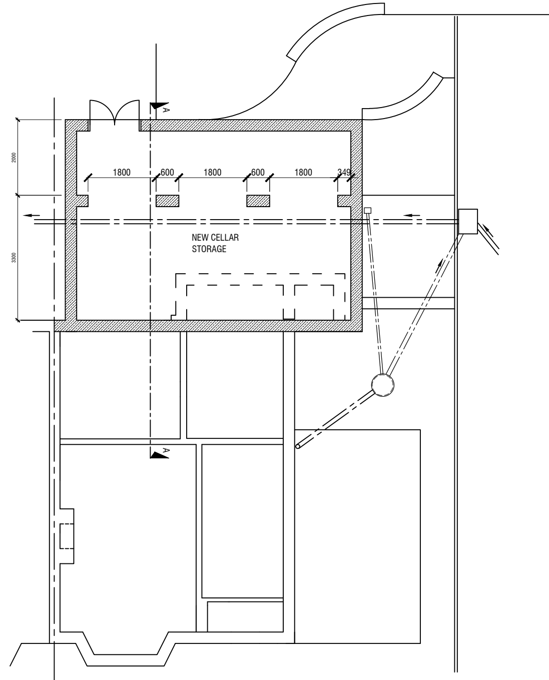
PROPOSED CELLAR STORAGE
