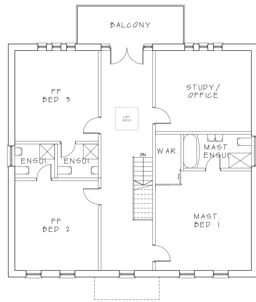
PROPOSED FIRST FLOOR Scale 1:100@A1
