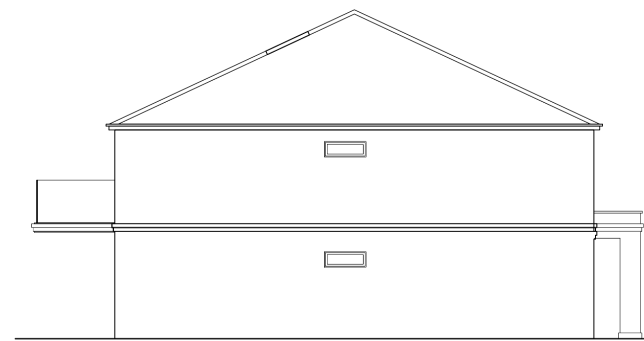
PROPOSED SIDE ELEV. Scale 1:100@A1
