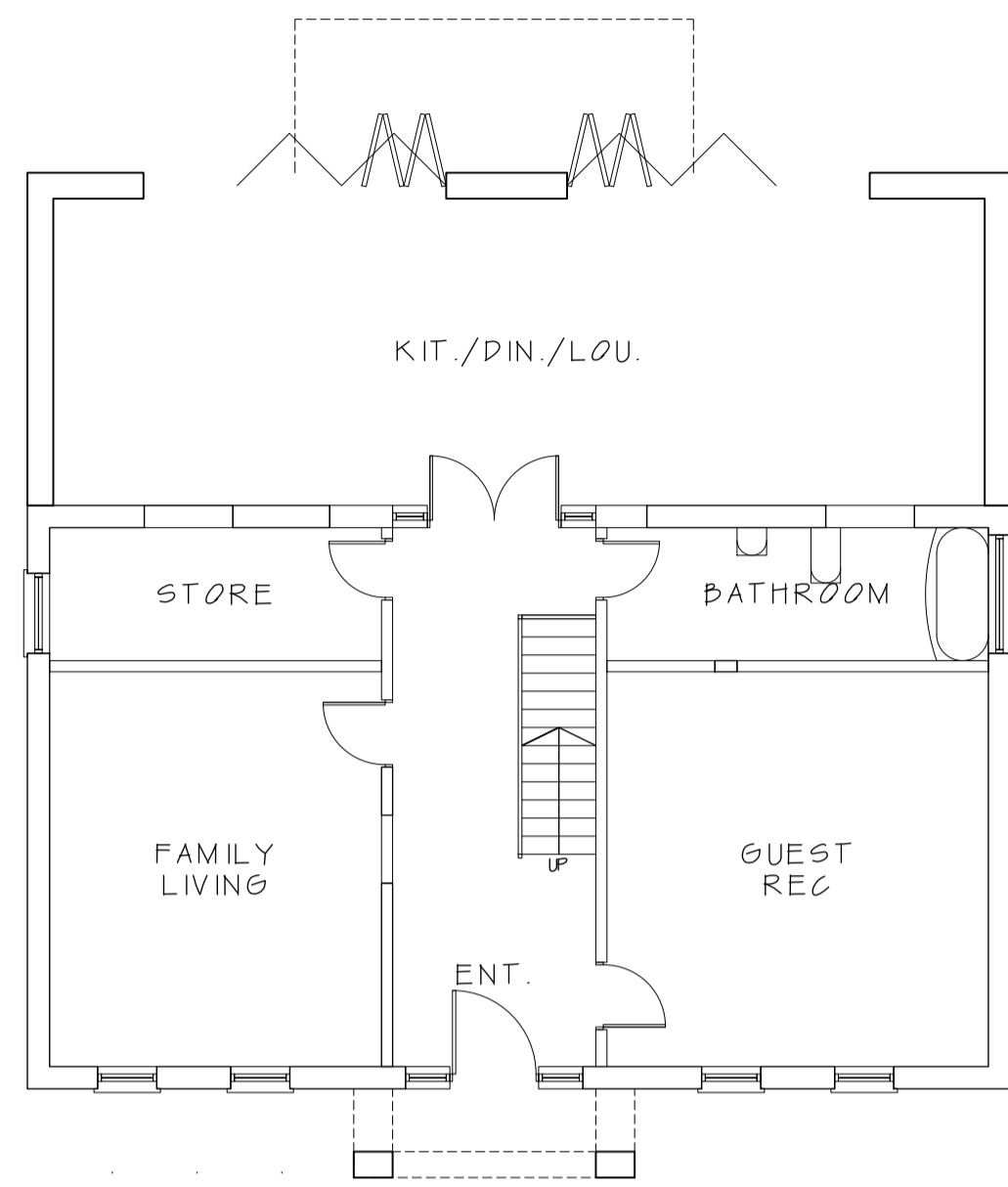
PROPOSED GROUND FLOOR Scale 1:100@A1
