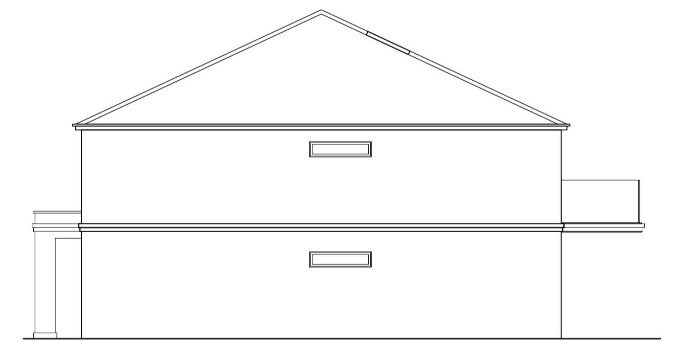
PROPOSED OTHER SIDE ELEV. Scale 1:100@A1
