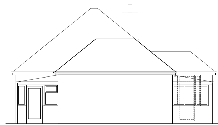
EXISTING SIDE ELEV. Scale 1:100@A1
