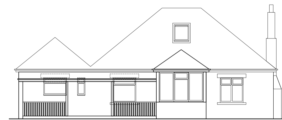
EXISTING REAR ELEV. Scale 1:100@A1
