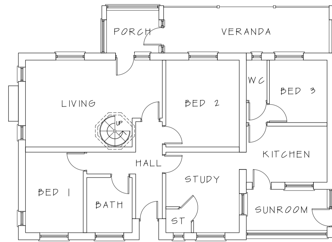
EXISTING GROUND FLOOR Scale 1:100@A1
